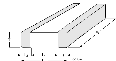
Fig. 2 Surface mounted multilayer ceramic capacitor dimension
