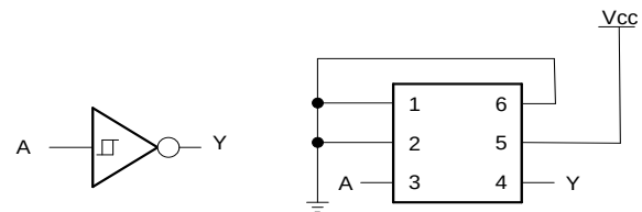
Configuration 6 Inverter
