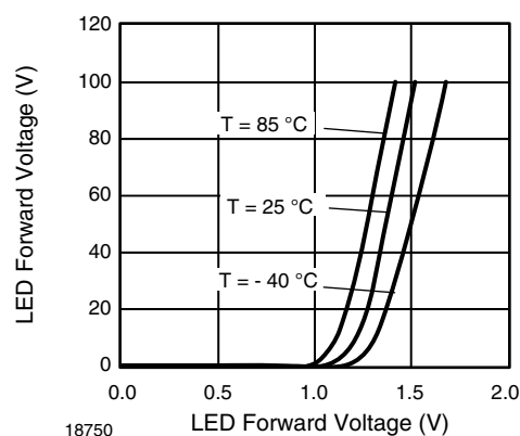
Fig. 3 - LED Forward Current vs. LED Forward Voltage
