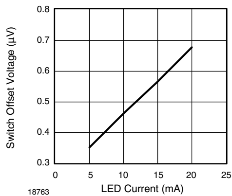
Fig. 16 - Switch Offset Voltage vs. LED Current
