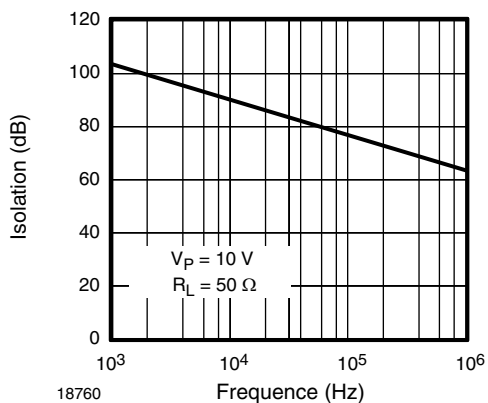
Fig. 13 - Output Isolation
