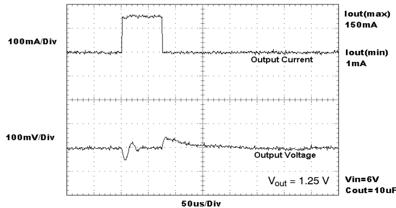
Figure 33. Load Transient Response ( 10 \mu F )
