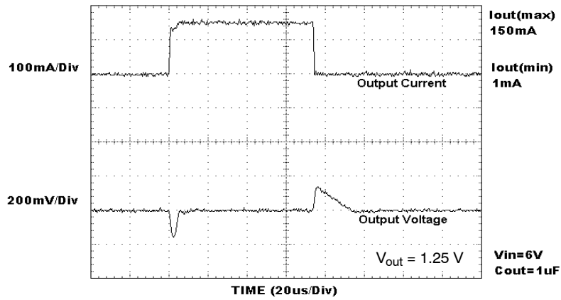
Figure 32. Load Transient Response ( 1.0 \mu F )
