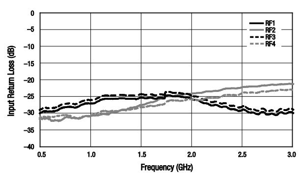
Figure 8. Input Return Loss vs Frequency
