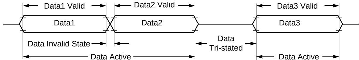
Figure 10-3 Signal States
