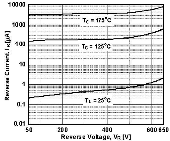
Figure 20. Reverse Current
