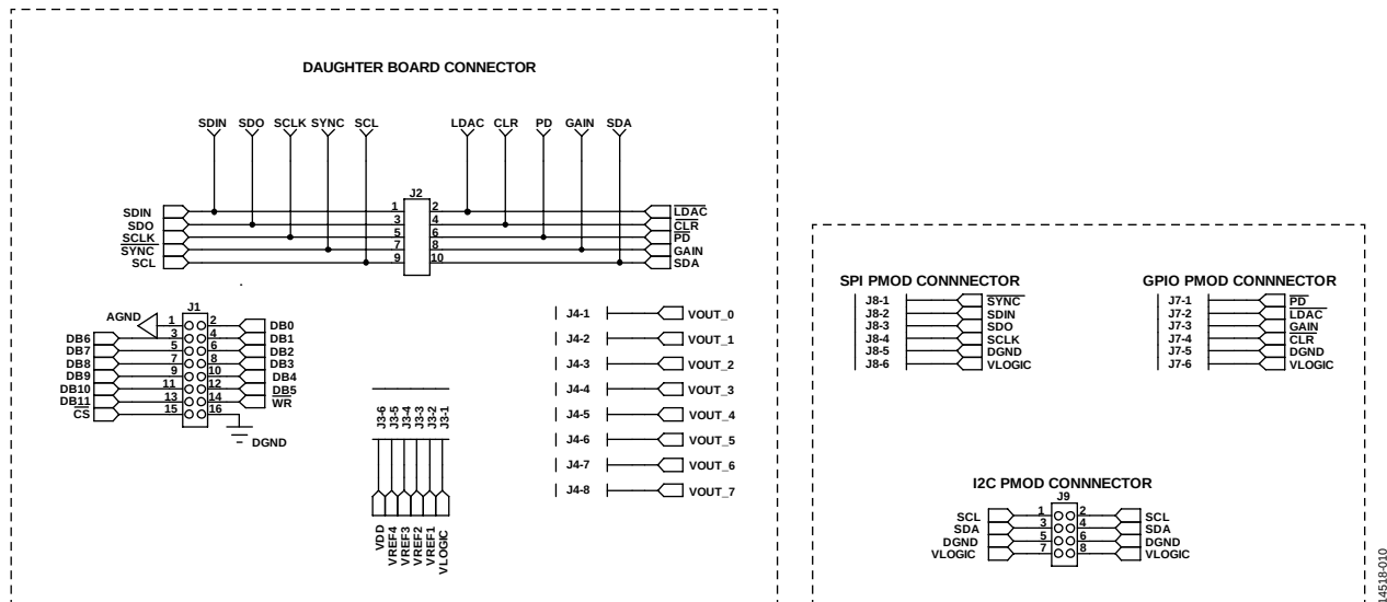
Figure 10. EVAL-MBnanoDAC-SDZ Motherboard Connectors to EVAL-AD5342DBZ Daughter Board and Serial Interface
