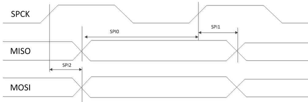
Figure 3 SPI Timing Diagram – Master Mode
