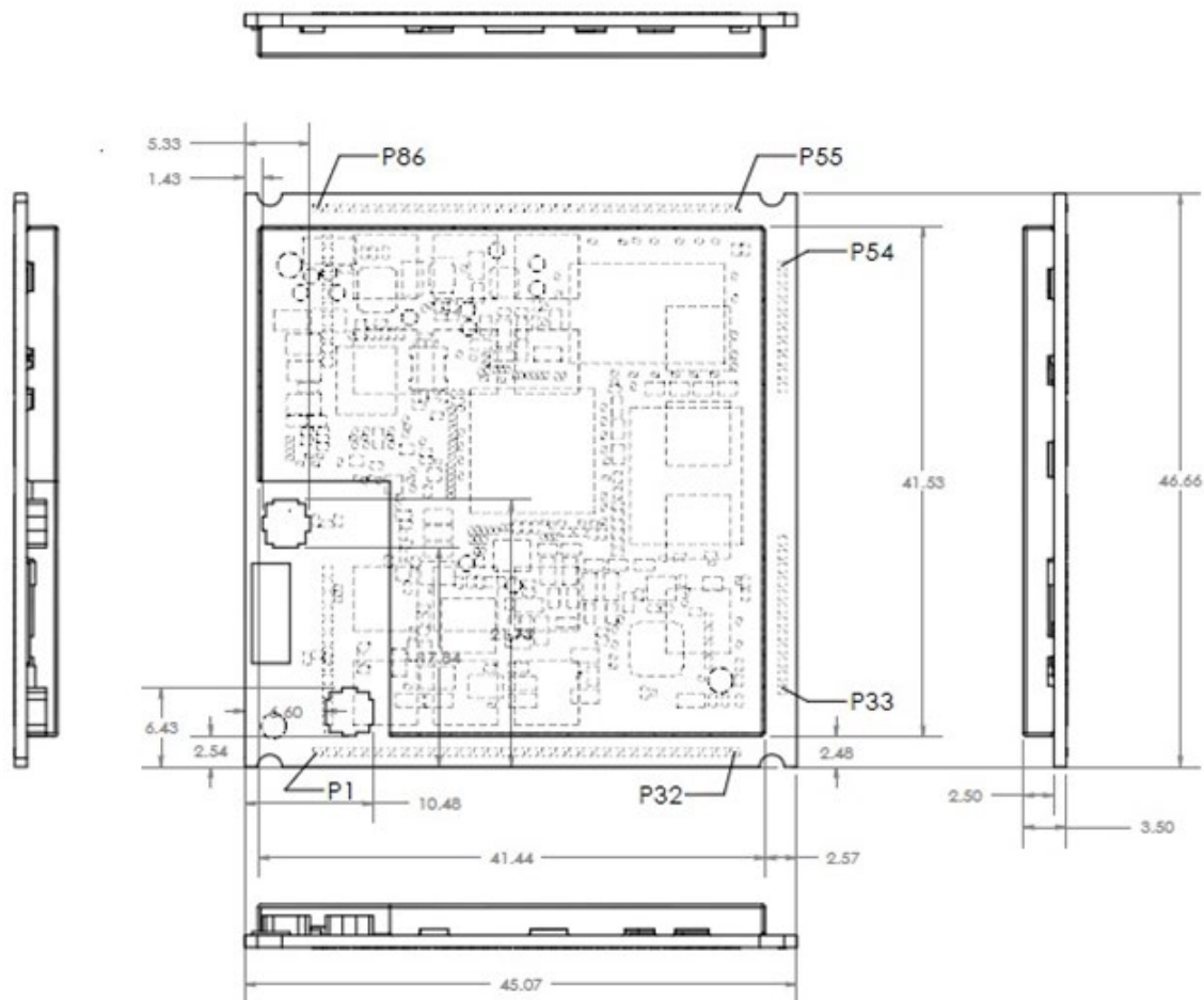
Figure 10 PW20502 Enterprise Wi-Fi IoT Wi-Fi Module
