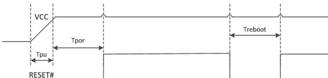
Figure 6 Reset Timing
