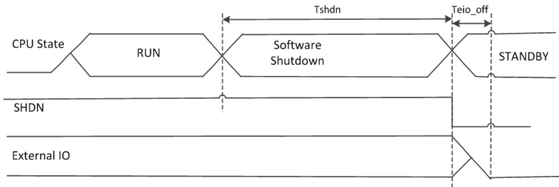
Figure 9 Shutdown Pin Timing
