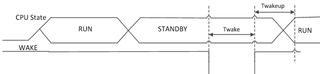
Figure 8 Wake Timing
