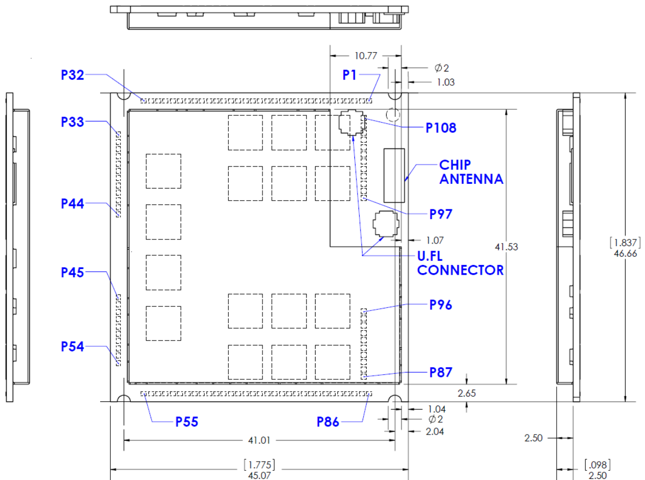
Figure 2 PremierWave 2050 Pad and Antenna Port Locations
