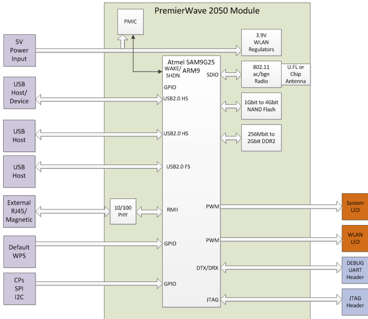
Figure 1 PremierWave 2050 Block Diagram
