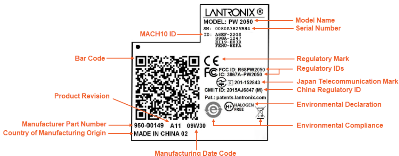
Figure 12 PremierWave 2050 Module Label
