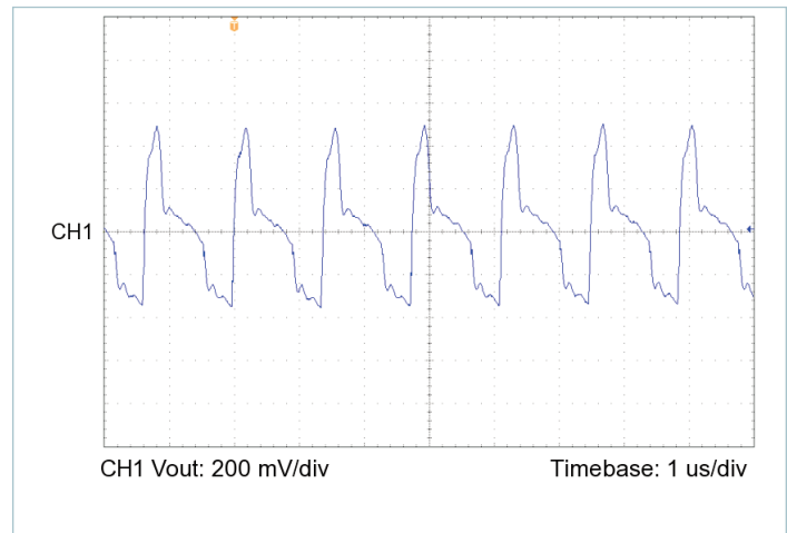
Figure 19 — Output voltage ripple, V_{IN} = 30\text{ V} , V_{OUT} = 48.0\text{ V} , C_{OUT\_EXT} = 200\text{ μF} , R_{LOAD} = 14.118\text{ Ω}
