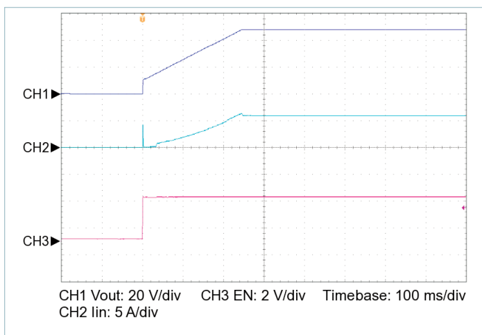
Figure 17 — Startup from EN, V_{IN} = 30\text{ V} , C_{OUT\_EXT} = 2000\text{ μF} , R_{LOAD} = 14.118\text{ Ω}
