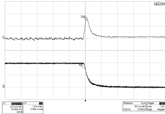
Figure 9. Load transient 2.0 A to 0.2 A, with V_{OUT} = 3.3 V and V_{IN} = 13.2 V
