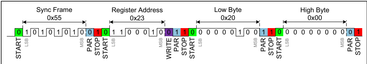
Figure 9: Example of WRITE (Reg[0x23] = 0x20 and Reg [0x24] = 0x00)
