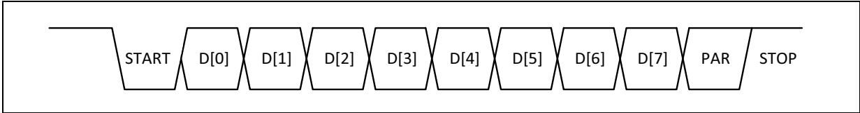
Figure 8: UART protocol frame
