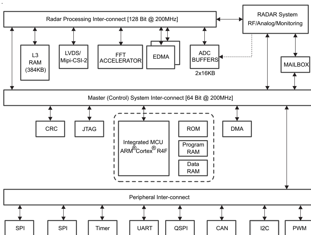
Figure 6-1. System Interconnect
