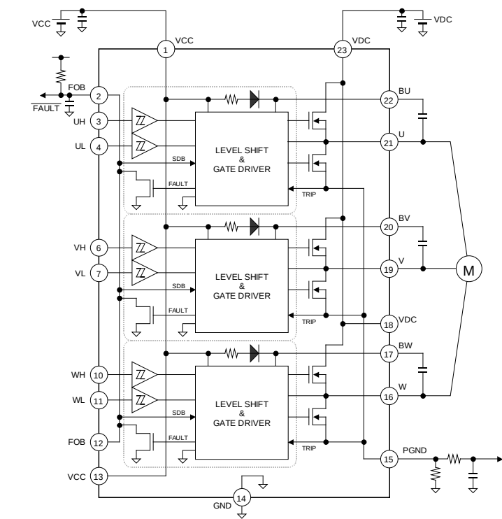
Figure 2. Block diagram
