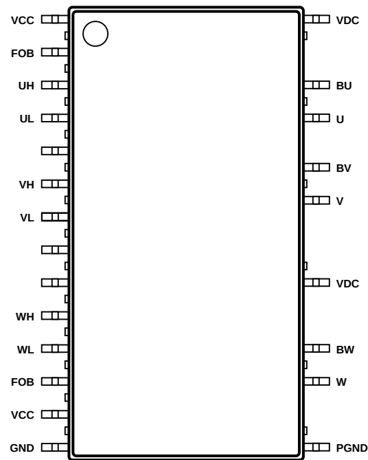
Figure 3. Pin configuration
