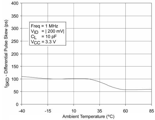
Figure 33. Differential Skew ( t_{PLH} - t_{PHL} ) vs. Ambient Temperature
