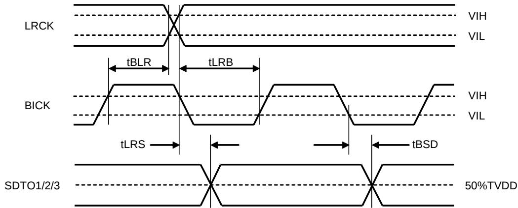
Figure 19. Audio Interface Timing (Normal Mode & Slave Mode: 8 kHz ≤ fs ≤ 216 kHz)
