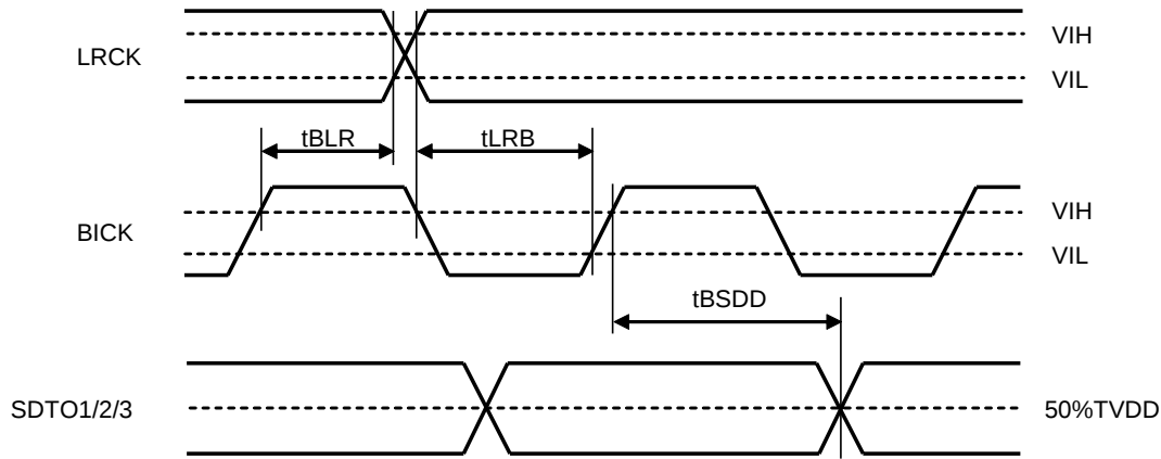
Figure 20. Audio Interface Timing (Normal & Slave Mode: fs=384 kHz, 768 kHz)
