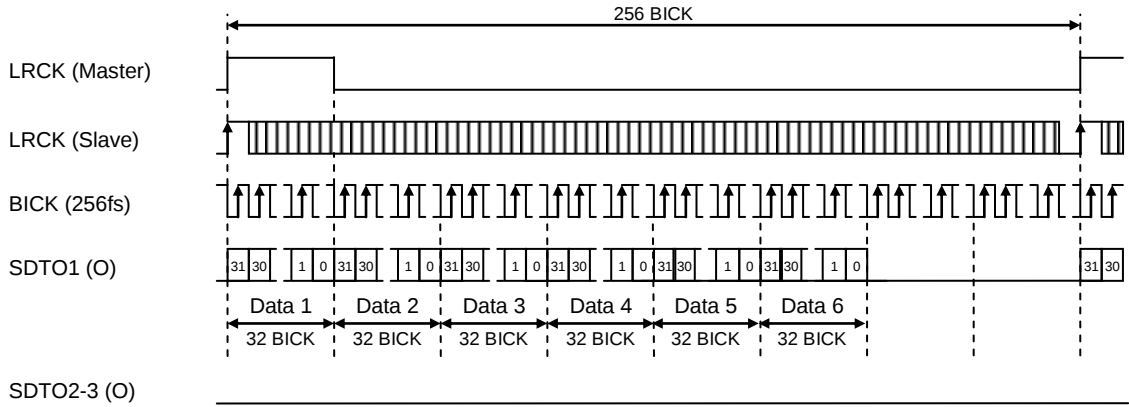
Figure 48. Mode 34/38 Timing (TDM256 Mode, MSB Justified, 32-bit)
