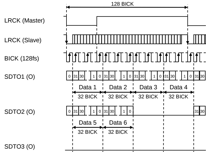
Figure 45. Mode 27/31 Timing (TDM128 Mode, I²S Compatible)
