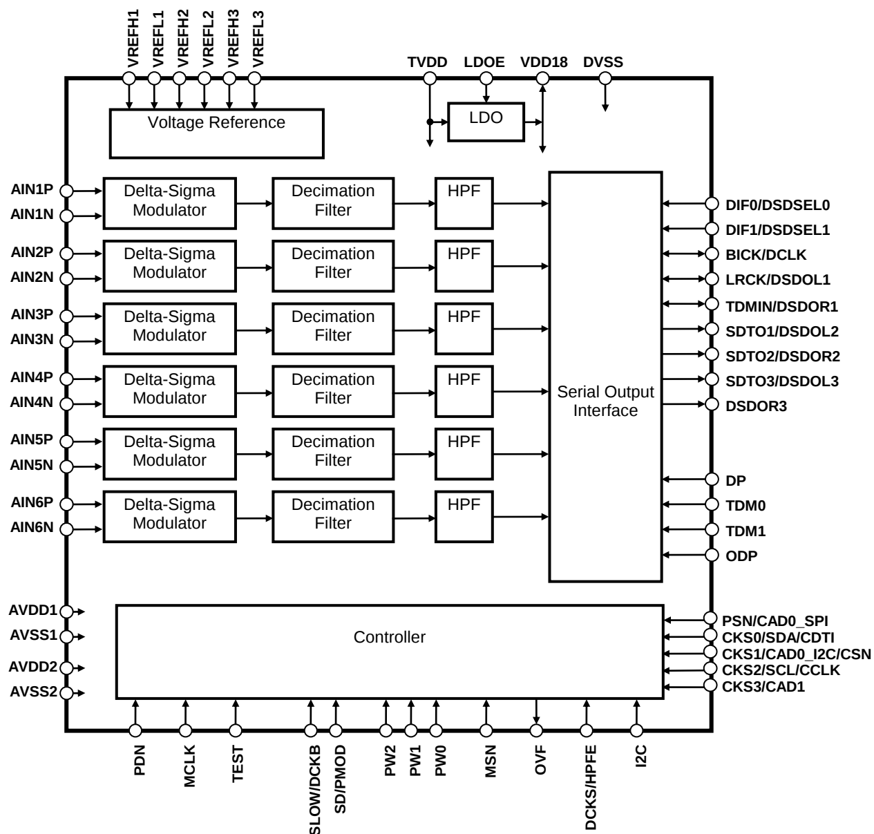
Figure 1. Block Diagram
