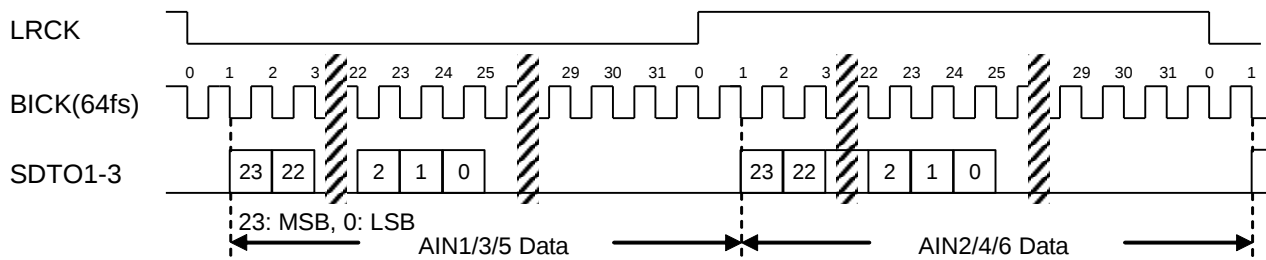
Figure 31. Mode 1/5 Timing (Normal Output, Normal/Double/Quad Speed Mode, I²S Compatible, 24-bit)
