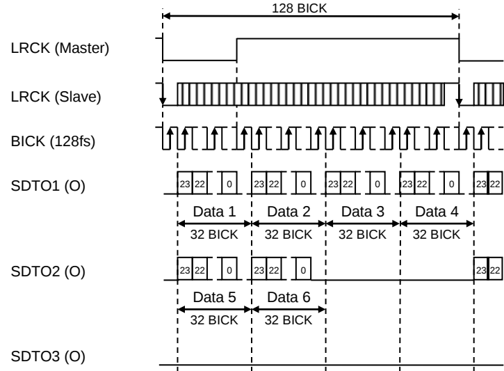
Figure 43. Mode 25/29 Timing (TDM128 Mode, I²S Compatible)
