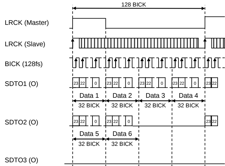
Figure 42. Mode 24/28 Timing (TDM128 Mode, MSB Justified, 24-bit)
