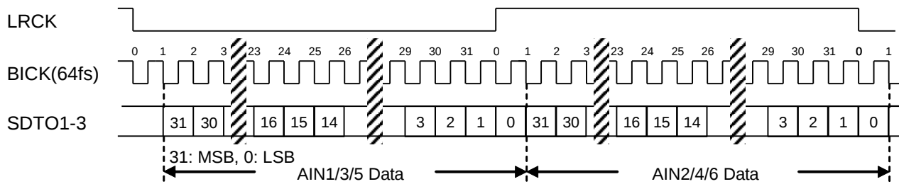
Figure 33. Mode 3/7 Timing (Normal Output, Normal/Double/Quad Speed Mode, I²S Compatible, 32-bit)
