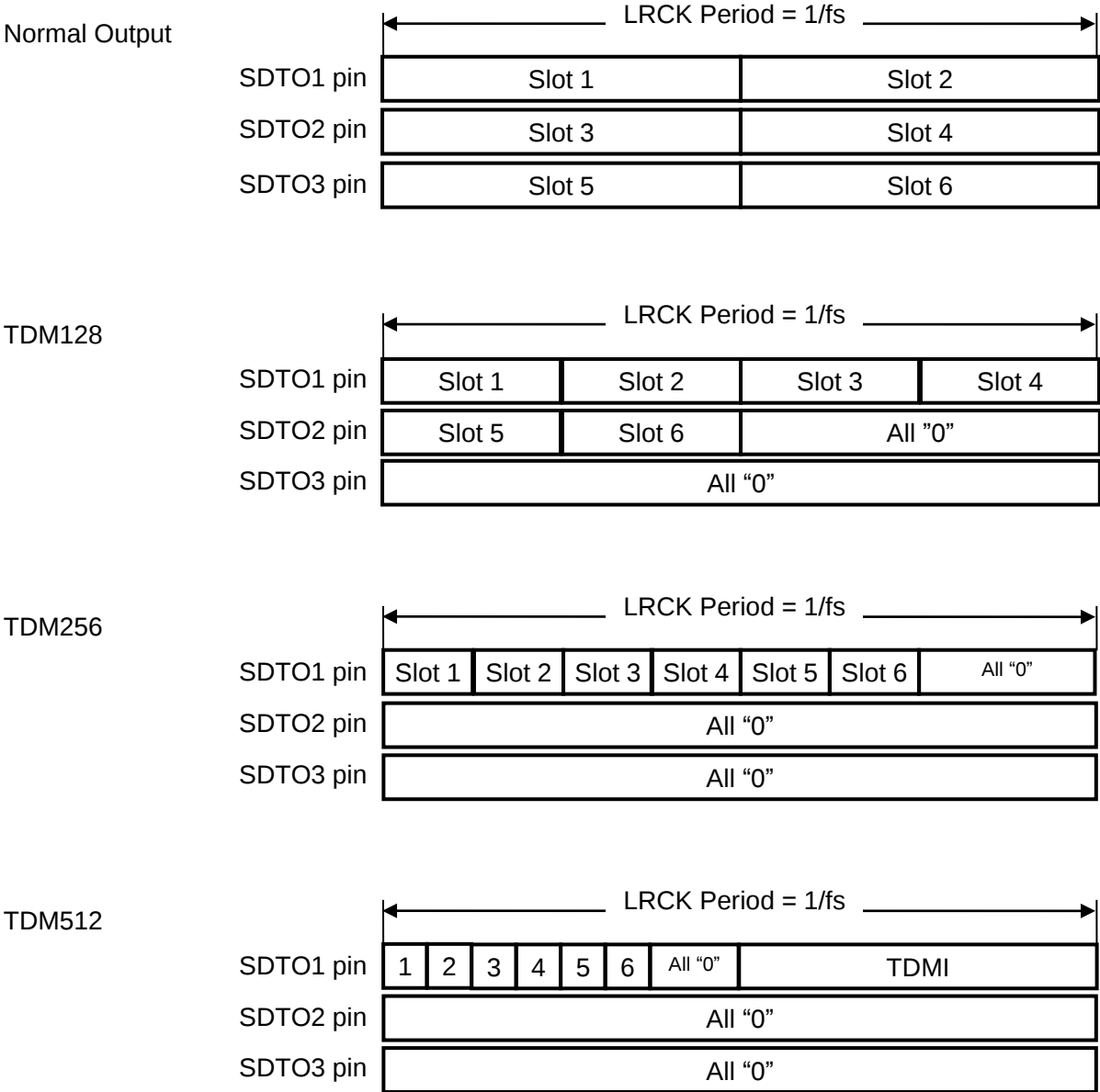
Figure 57. Slot Assign in PCM Mode
