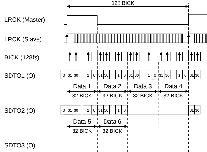
Figure 44. Mode 26/30 Timing (TDM128 Mode, MSB Justified)
