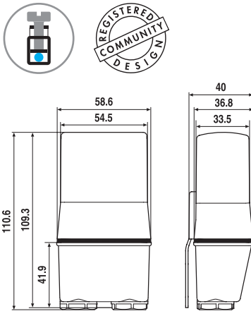
Type 10.32/10.41/10.42 Box clamp
