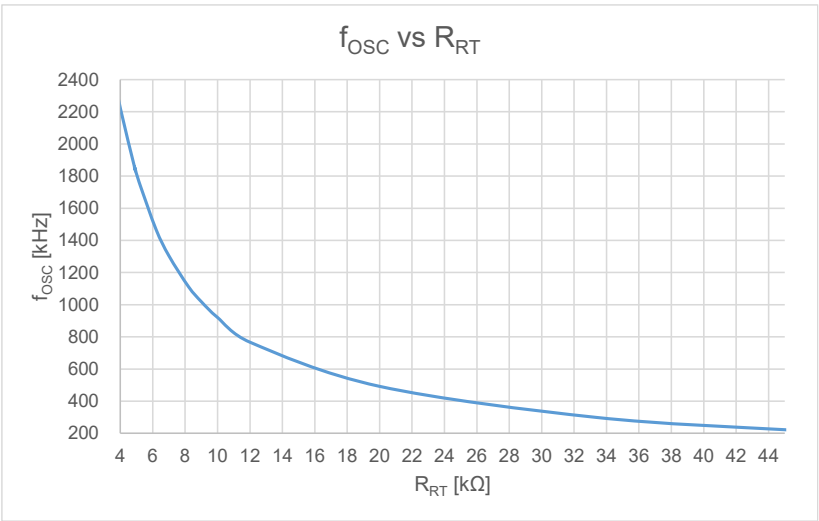
Figure 21. fosc vs RRT
