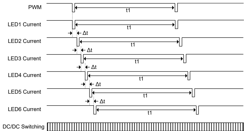
Figure 16. Phase Delay Operation for PWM Max Duty
