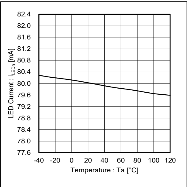
Figure 7. LED Current vs Temperature ( R_{SET} = 31.2\text{ k}\Omega , n = 1 to 6)
