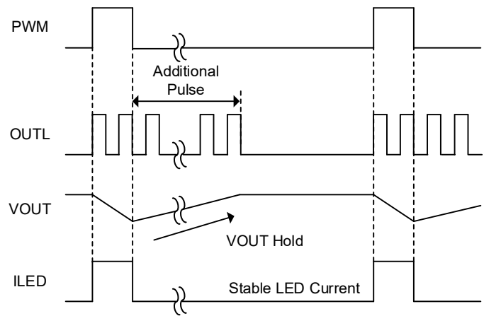
Figure 22. Pulse Addition Function
