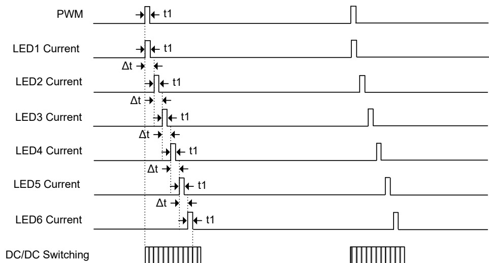
Figure 15. Phase Delay Operation for PWM Min Duty
