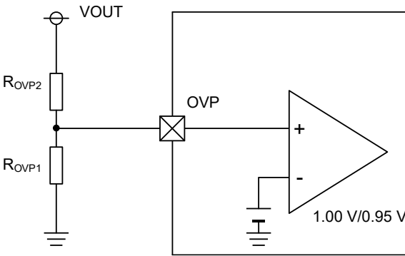
Figure 20. OVP Peripheral Circuit Diagram
