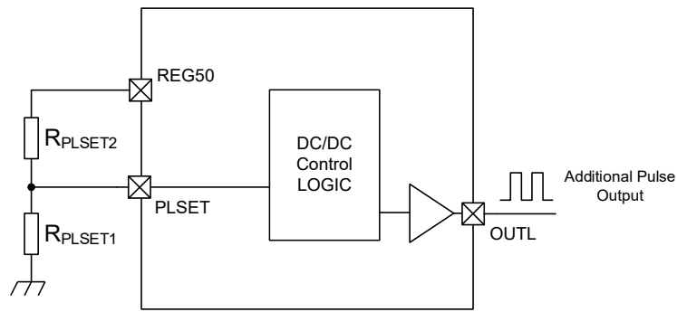
Figure 23. Additional Pulse Number Setting Method
