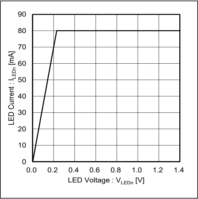
Figure 6. LED Current vs LED Voltage ( T_a = 25\text{ }^{\circ}\text{C} , R_{SET} = 31.2\text{ k}\Omega , n = 1 to 6)
