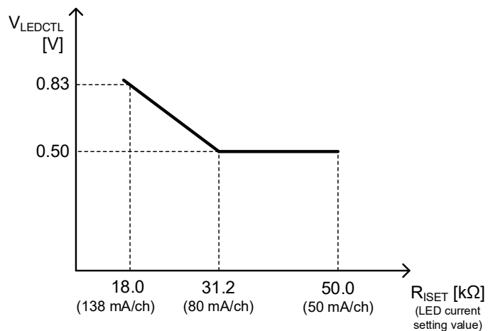
Figure 19. Relation Between LED Pin Control Voltage ( V_{\text{LEDCTL}} ) and R_{\text{SET}}
