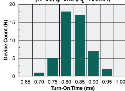
Typical Turn-On Time (N=50, I_F=5\text{mA} , I_L=130\text{mA} )
