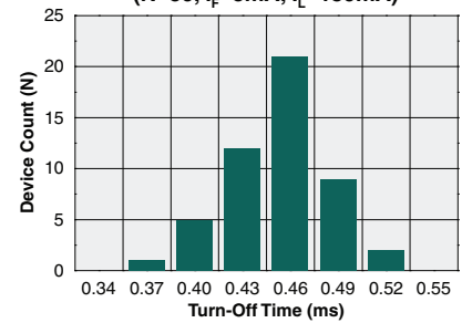
Typical Turn-Off Time (N=50, I_F=5\text{mA} , I_L=130\text{mA} )
