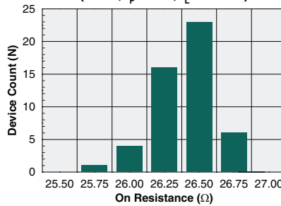
Typical On-Resistance Distribution (N=50, I_F=2\text{mA} , I_L=130\text{mA} )
