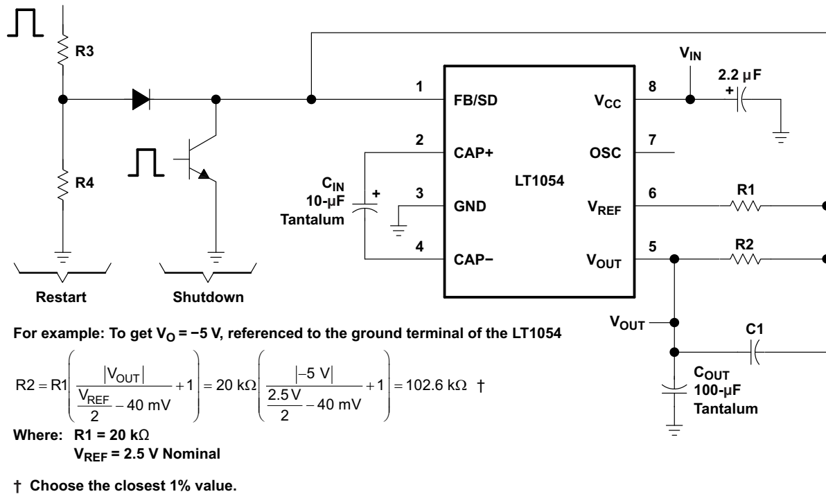
Figure 11. Basic Regulation Configuration
