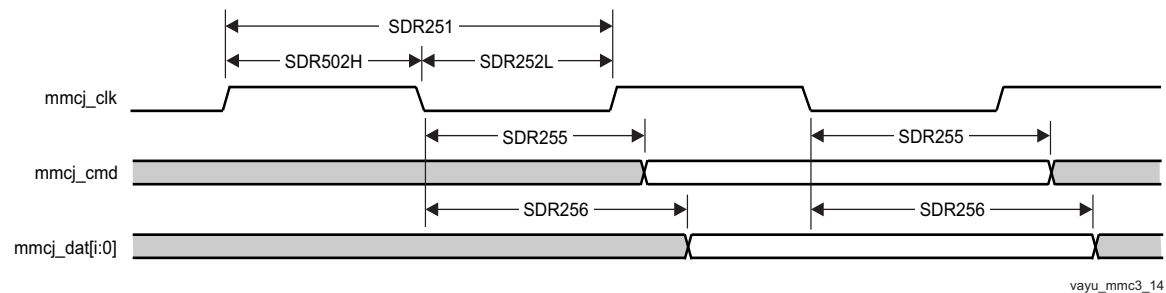
Figure 5-105. MMC/SD/SDIOj in - SDR25 - Transmitter Mode
