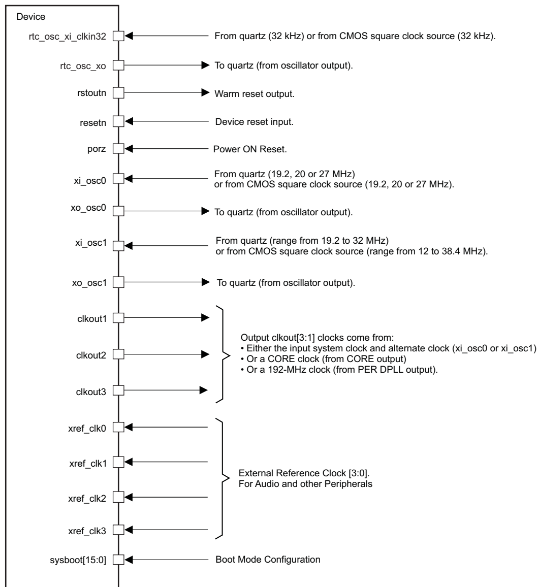
Figure 5-8. Clock Interface
