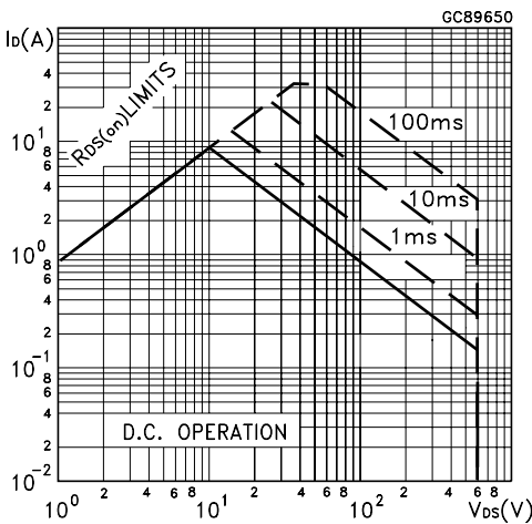
Safe Operating Area for ISOWATT218
