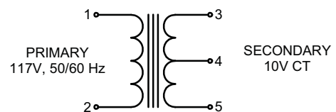
SCHEMATIC DIAGRAM
