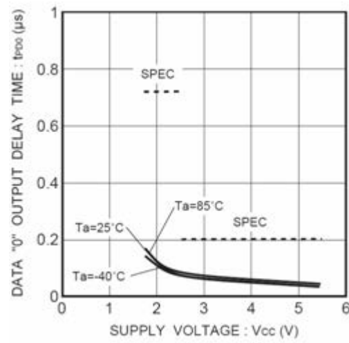
Figure 27. Data "0" output delay time t_{PD0}
