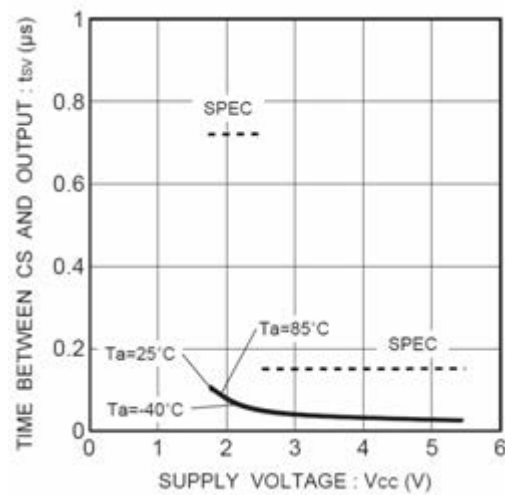
Figure 29. Time from CS to output establishment t_{SV}
