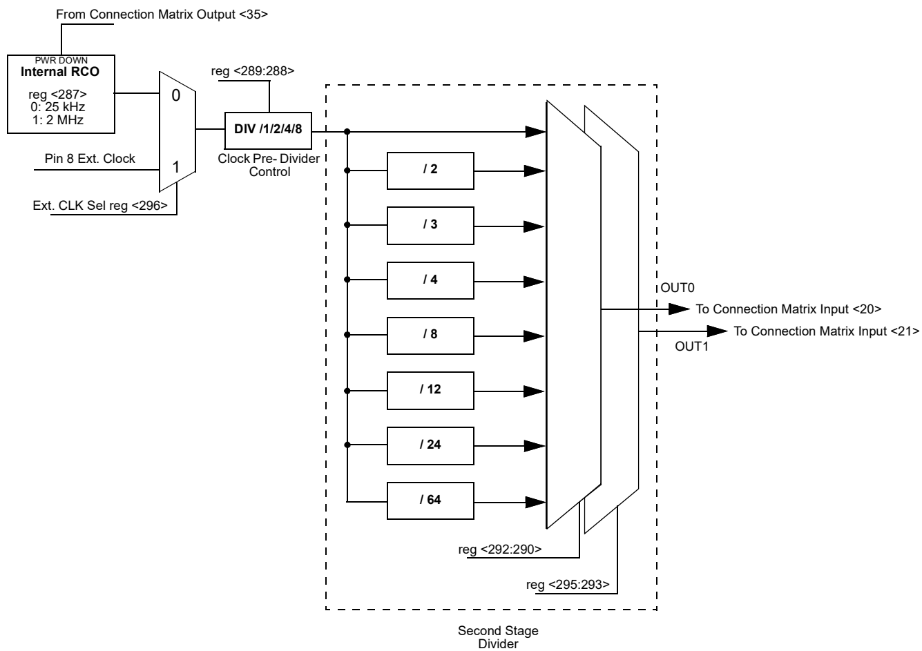
Figure 31. RC OSC Block Diagram
