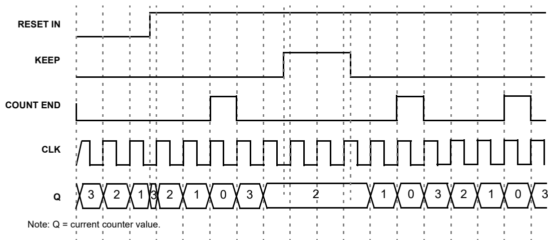
Figure 20. Timing (Set Rising Edge Mode, Oscillator is Forced On, UP = 0) for Count Data = 3
