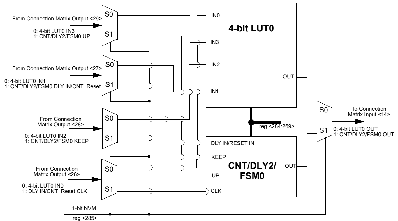
Figure 15. 4-bit LUT1 or CNT/DLY2/FSM0
