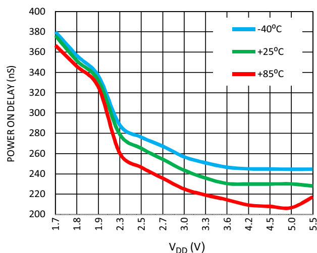
Figure 29. Maximum Power-On Delay vs. V_{DD} , RC OSC = 2 MHz
