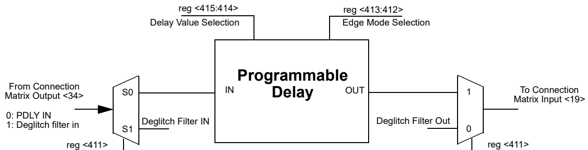
Figure 23. Programmable Delay
