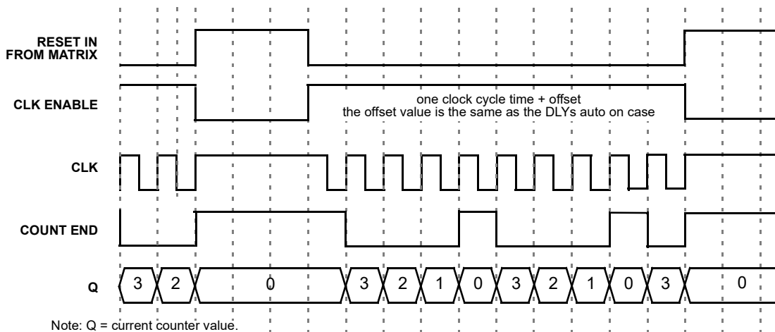
Figure 18. Timing (Reset High Level Mode, Oscillator is Auto Powered On (Controlled by Reset)) for Count Data = 3
