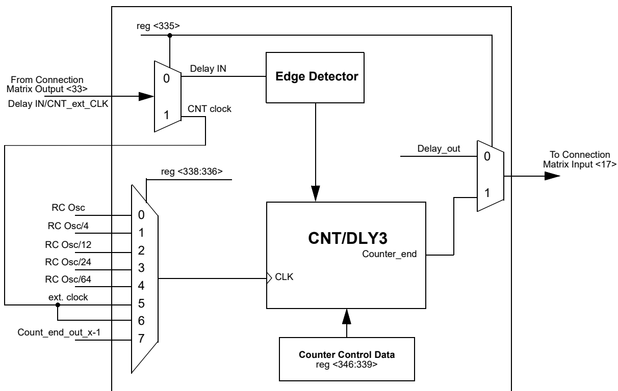
Figure 28. CNT/DLY3
