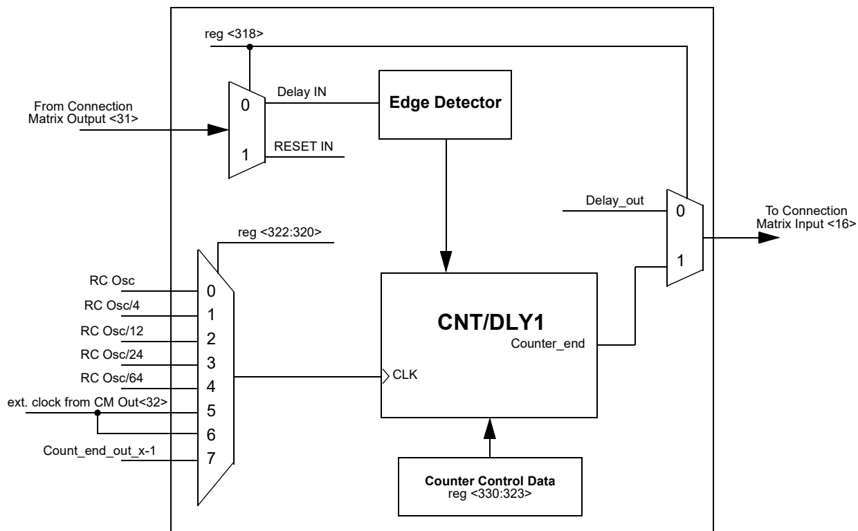
Figure 27. CNT/DLY1
