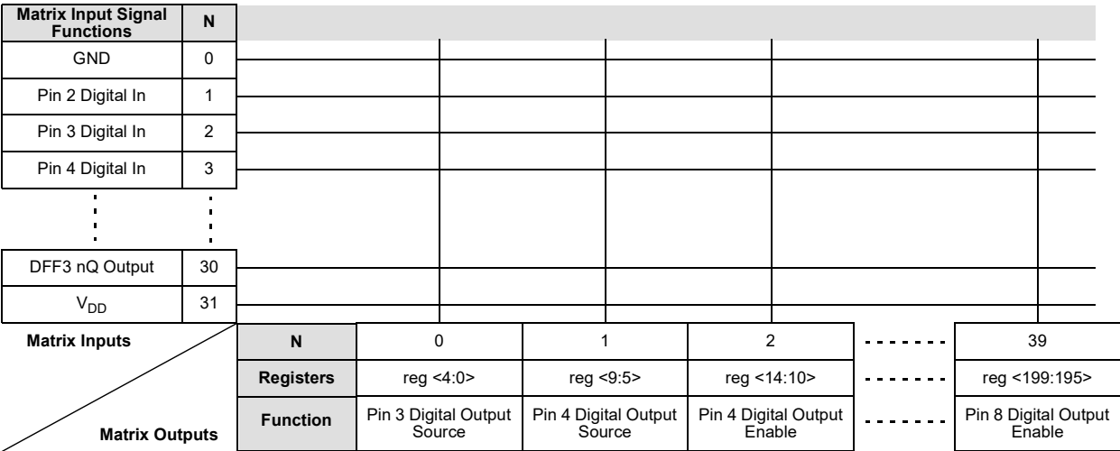
Figure 6. Connection Matrix
