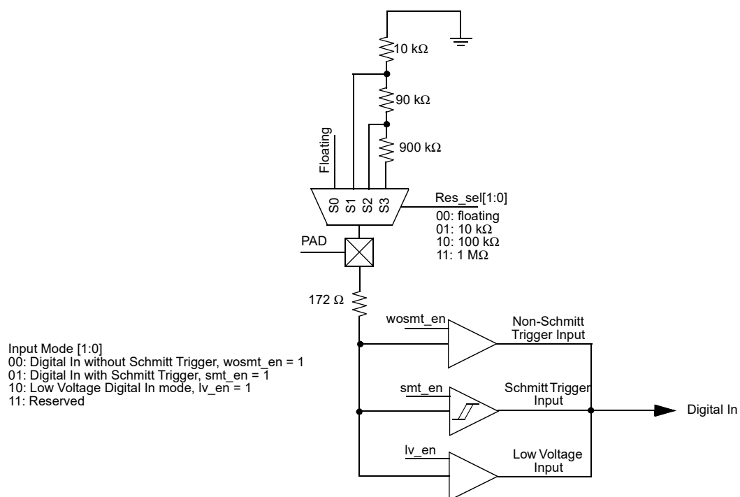
Figure 3. Pin 2 GPI IO Structure Diagram
