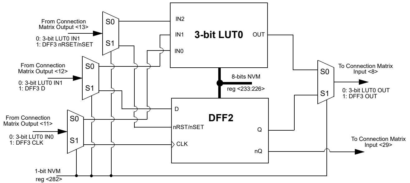
Figure 12. 3-bit LUT0 or DFF2
