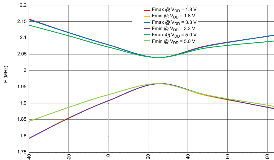
Figure 32. RC Oscillator Frequency vs. Temperature, RC OSC = 2 MHz
