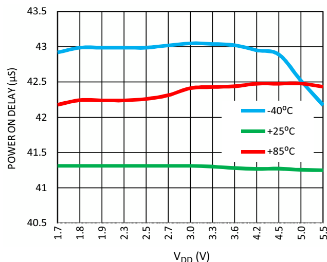
Figure 30. Maximum Power-On Delay vs. V DD , RC OSC = 25 kHz
