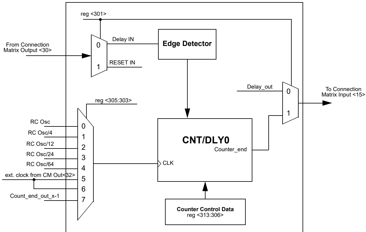
Figure 26. CNT/DLY0
