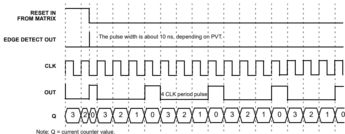
Figure 17. Timing (Reset Falling Edge Mode, Oscillator is Forced On) for Count Data = 3
