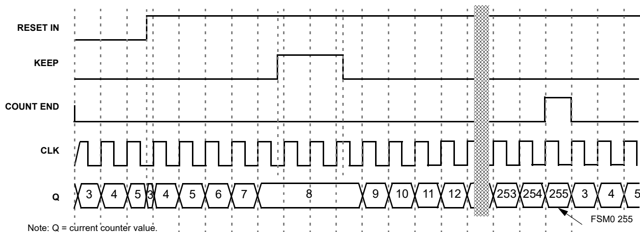
Figure 22. Timing (Set Rising Edge Mode, Oscillator is Forced On, UP = 1) for Count Data = 3
