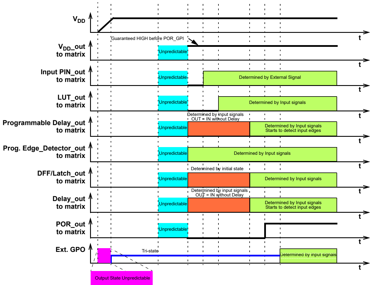
Figure 35. Internal Macrocell States during POR Sequence
