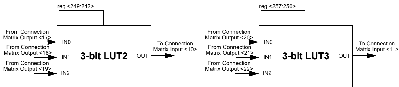
Figure 9. 3-bit LUTs
