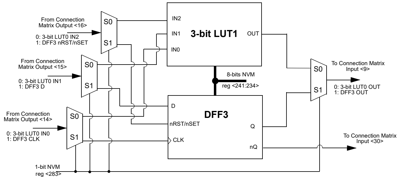
Figure 13. 3-bit LUT1 or DFF3
