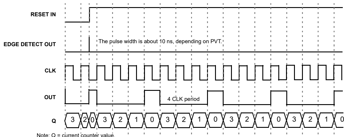
Figure 16. Timing (Reset Rising Edge Mode, Oscillator is Forced On) for Count Data = 3
