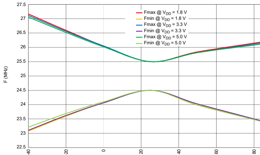
Figure 33. RC Oscillator Frequency vs. Temperature, RC OSC = 25 kHz
