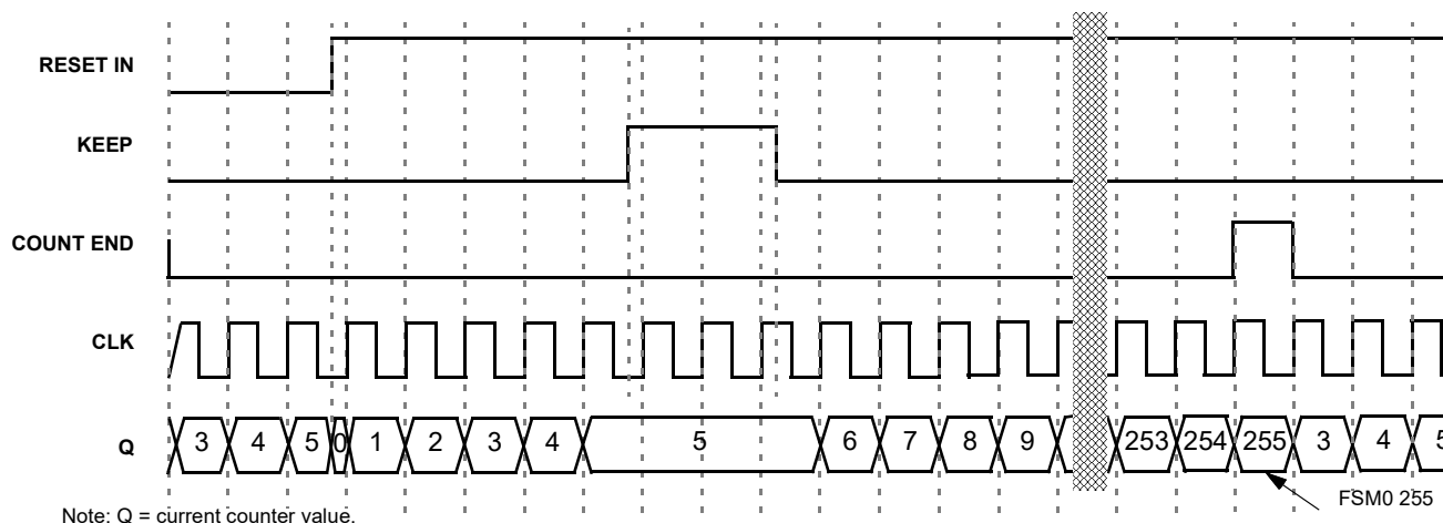
Figure 21. Timing (Reset Rising Edge Mode, Oscillator is Forced On, UP = 1) for Count Data = 3
