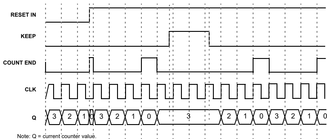
Figure 19. Timing (Reset Rising Edge Mode, Oscillator is Forced On, UP = 0) for Count Data = 3
