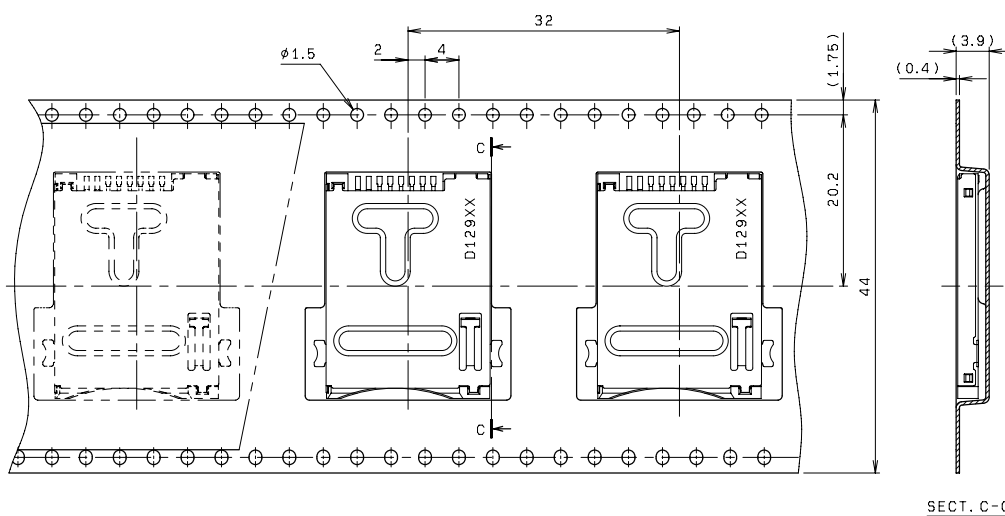
SECT. C-C
