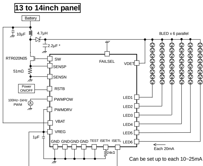
Figure 49. 8 series×6 parallel, LED current 20mA setting Power control PWM application;:n
