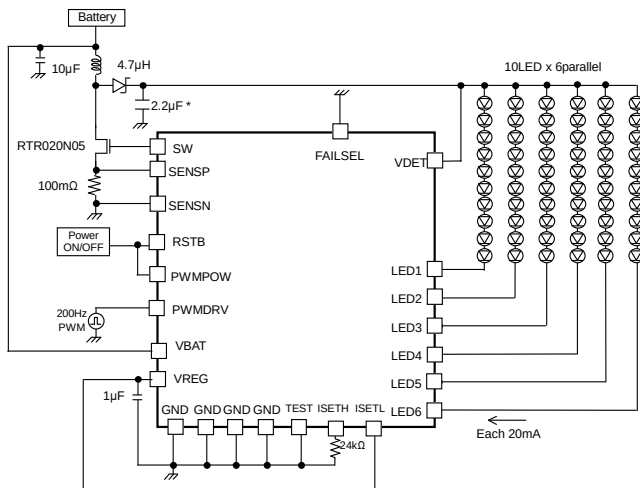
Figure 27. 10 series × 6parallel H current 20mA setting Current driver PWM application
