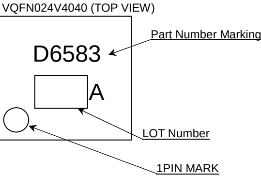
Figure 66. Marking Diagram
