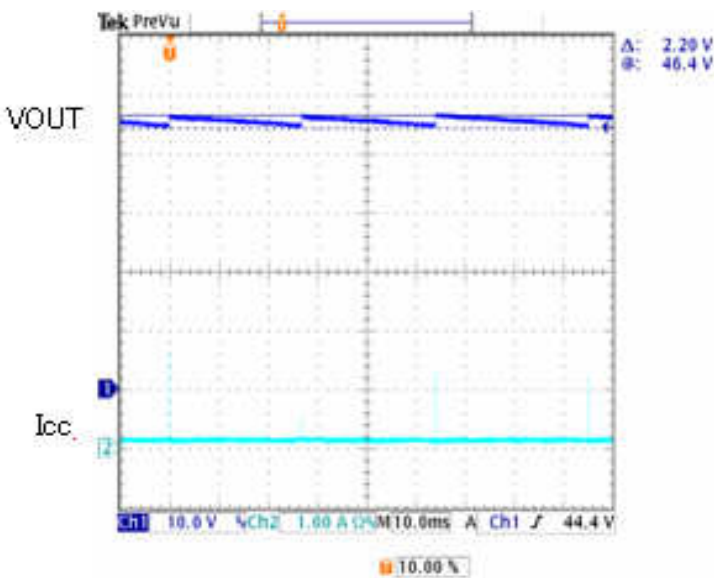
Figure 26. VOUT@OVP(LED OPEN)
