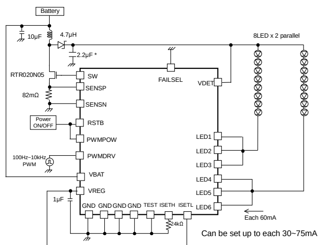
Figure 60. 8 series×2 parallel, LED current 60mA setting Current driver PWM application
