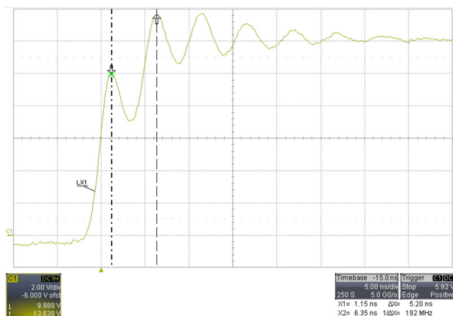
Figure 23: Typical LX ring frequency at turn-on without a snubber and V_{\text{VIN}} = 12 \text{ V} : f_{\text{RING}} = 192 \text{ MHz}
