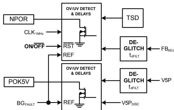
Figure 11: NPOR and POK5V Fault Outputs
