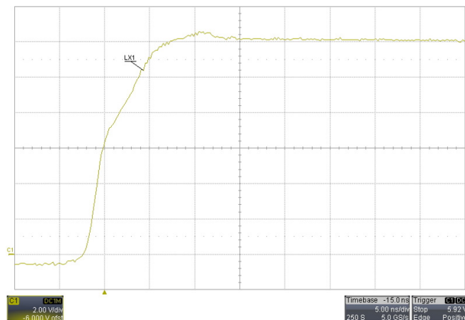
Figure 26: LX waveform including an RC snubber consisting of 8.66\ \Omega + 270\ \text{pF}
