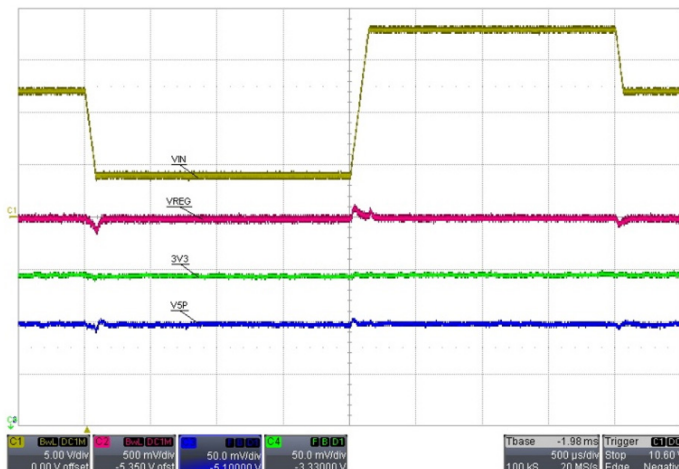
Figure 2: A4413 buck-boost operation at full load with V_{IN} slew rates of 100 V/ms; V5P deviates only \pm 0.14\% ( \pm 7\text{ mV} ).
