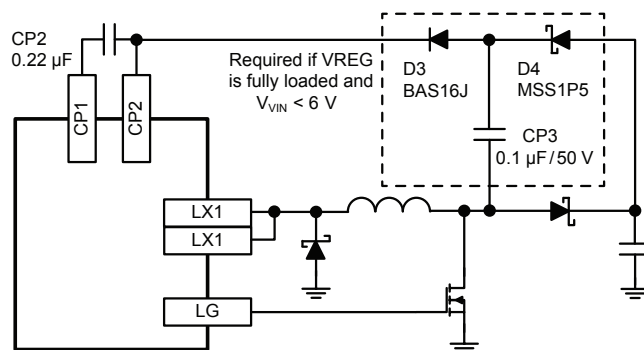
Figure 10: Charge pump enhancement components D3, D4, and CP3 are required if V_{VIN} < 6\ \text{V} .
