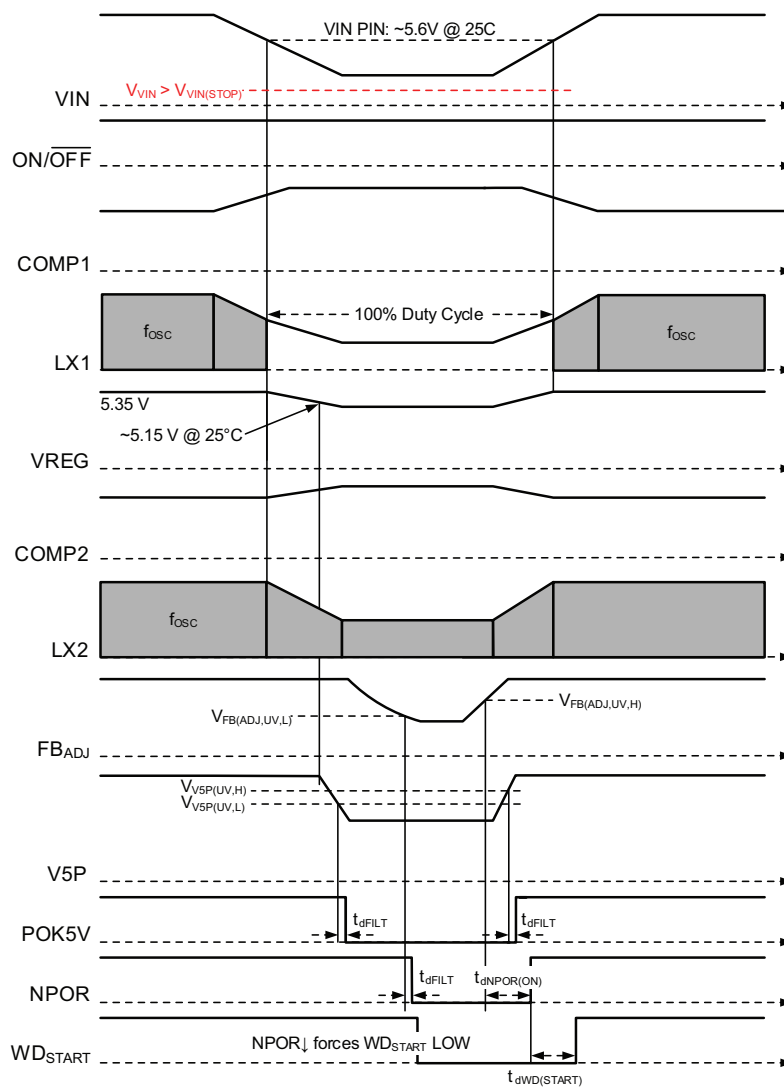
Figure 13: Buck Only Mode, Input Voltage (VIN) Undervoltage, V_{VIN} > V_{VIN(STOP)}
