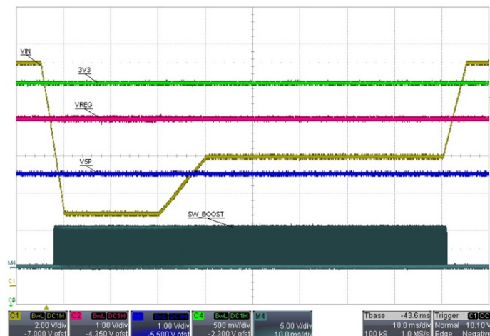
Figure 1: A4413 buck-boost operation at full load with V_{IN} slew rates ranging from 0.3 V/ms to 1.6 V/ms, representative of an automotive start/stop waveform.
