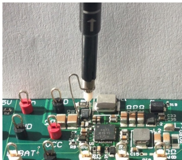
Figure 22: Measure LX ringing with tip-and-barrel
