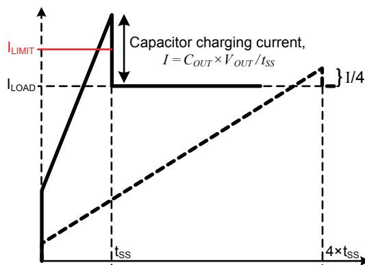
Figure 3: Capacitor charging currents versus soft-start time ( t_{SS1} ) when f_{OSC} and C_{OUT} are unchanged.
