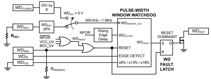
Figure 7: Pulse-Width Window Watchdog
