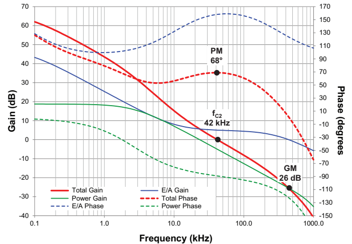
Figure 21: Bode Plot for the Synchronous Buck at 3.3 V OUT
