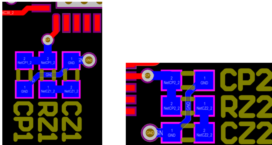
Figure 33b: Recommended placement and routing of COMP1 and COMP2 components.
