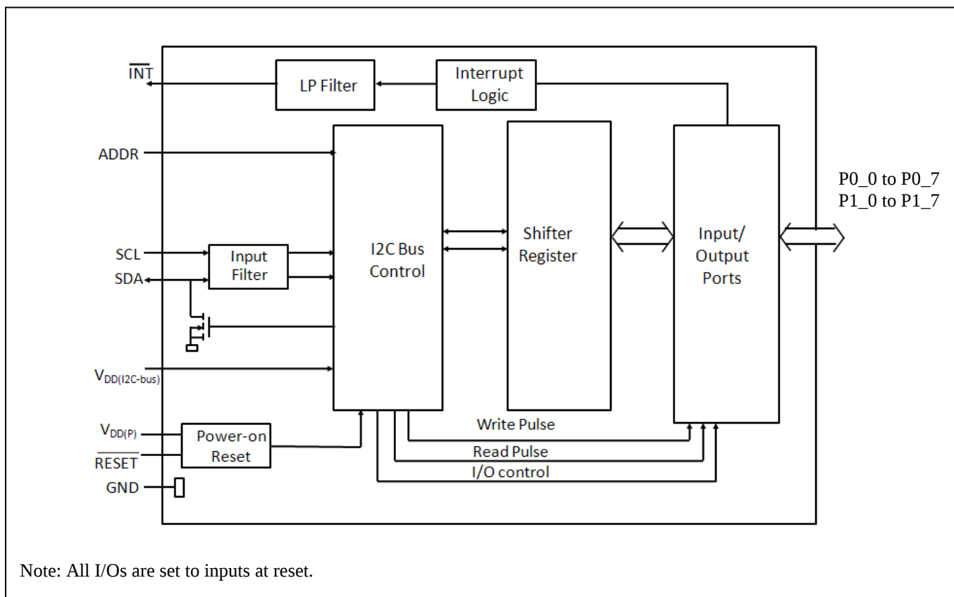
Fig7: Block diagram
