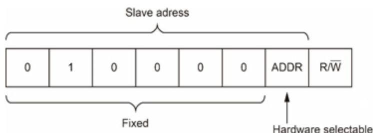
Fig. 10: PI4IOE5V6416 address
