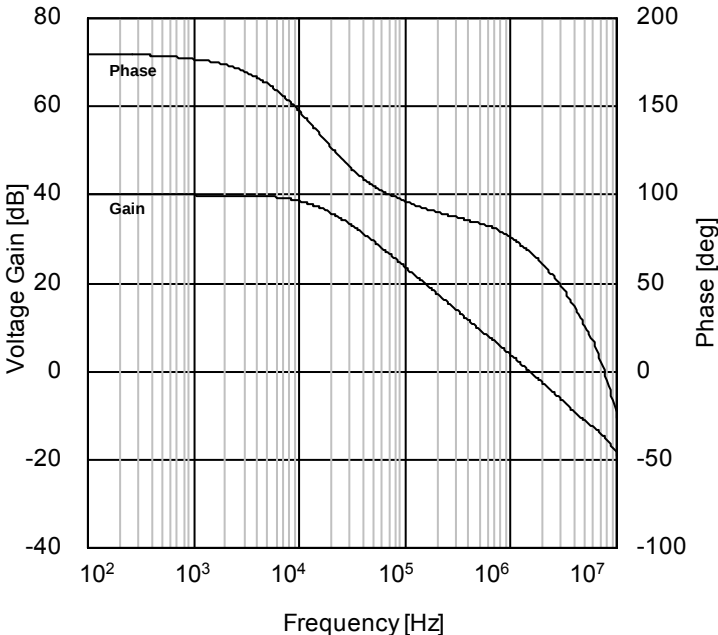
Figure 20. Voltage Gain · Phase vs Frequency ( V+=5V , R_L=2k\Omega , T_A=25^\circ C )
