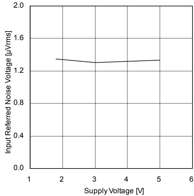
Figure 78. Input Referred Noise Voltage vs Supply Voltage ( T_A=25^{\circ}\text{C} )
