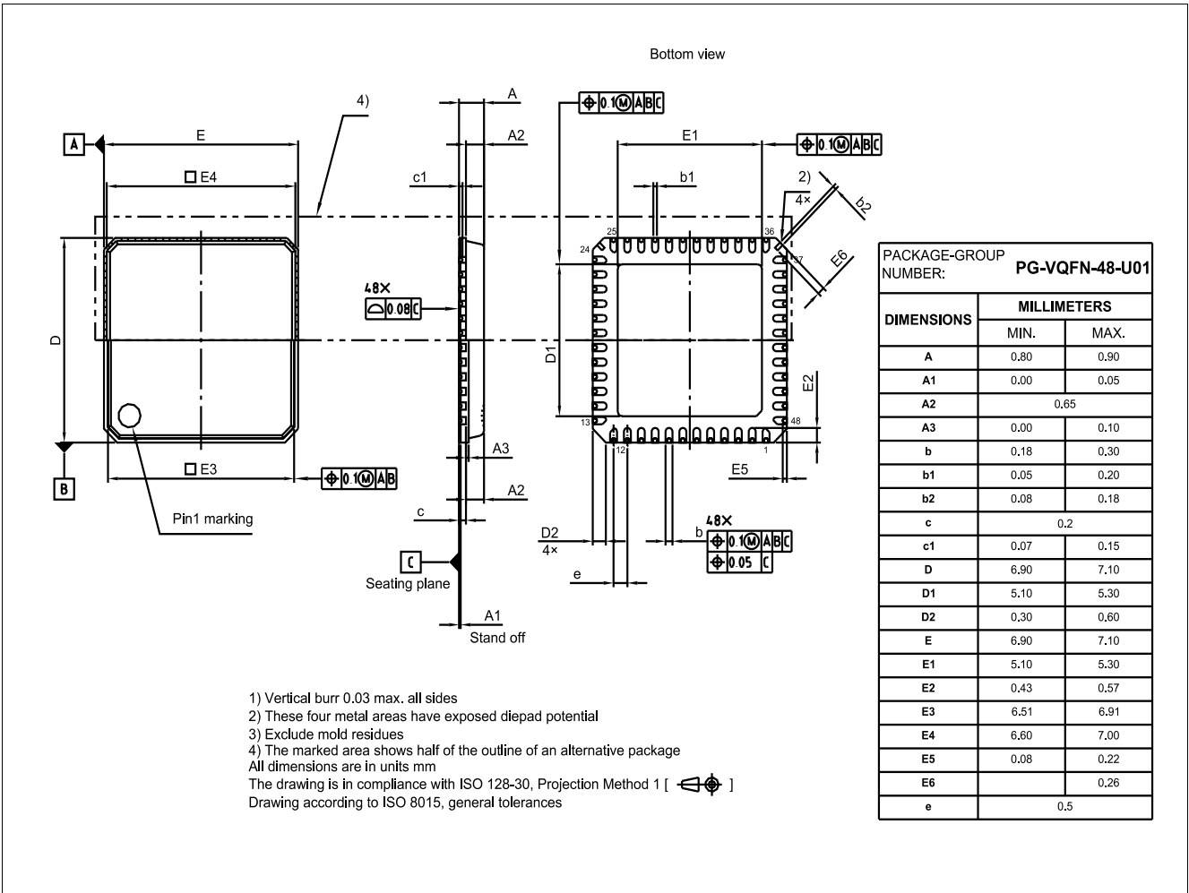
Figure 64 PG-VQFN-48 1)
