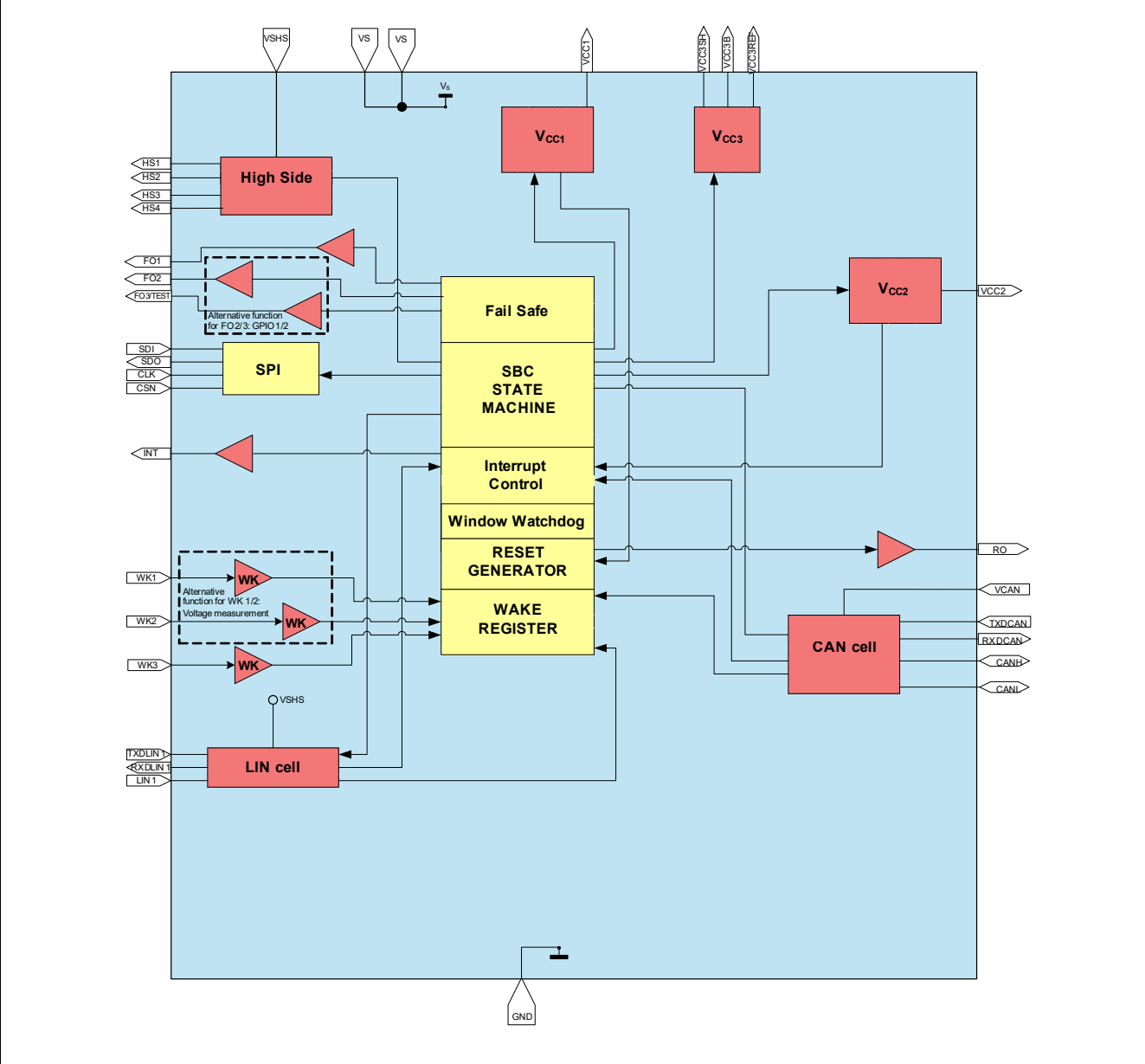
Figure 1 Block Diagram
