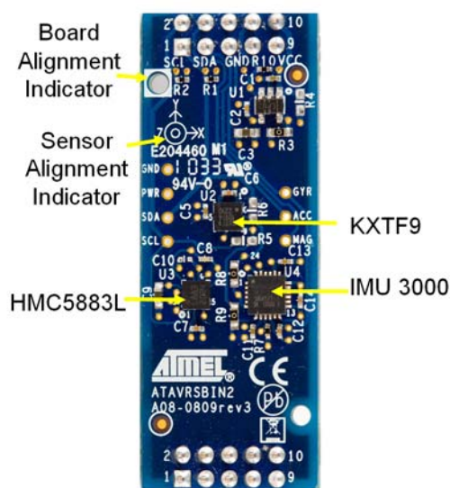
Figure 4-1. Sensor arrangement.
