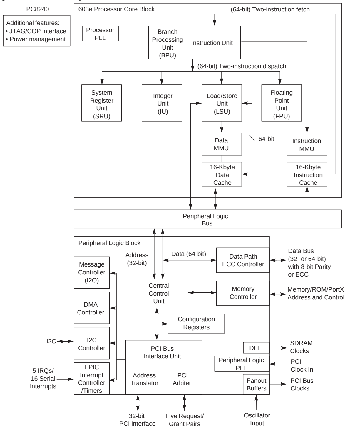
Figure 1-1. Block Diagram
