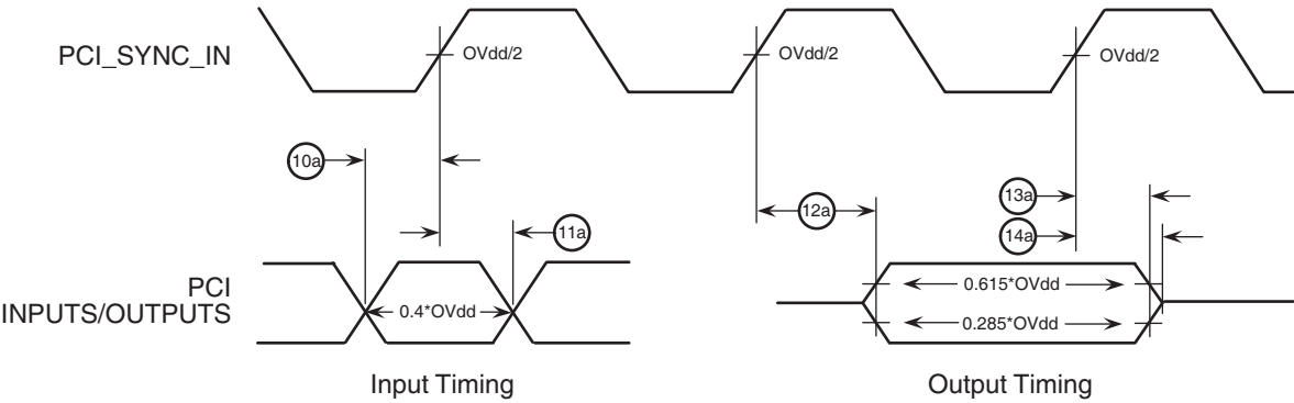
Figure 4-4. Input – Output Timing Diagram Referenced to PCI_SYNC_IN
