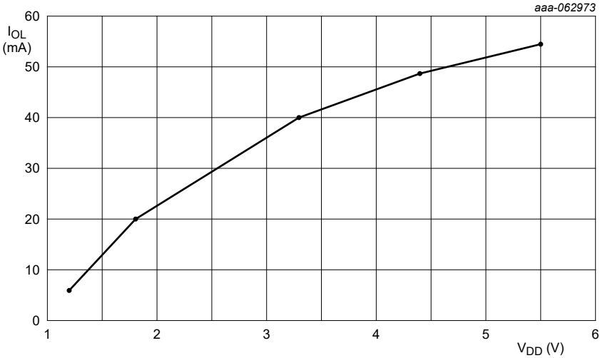
Figure 34. I_{OL} on pin \overline{SDA}/\overline{CE}
