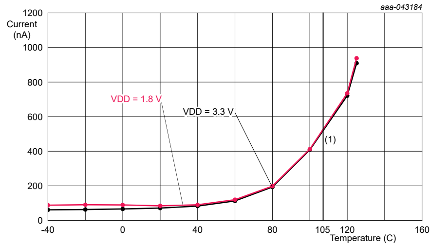
Figure 35. I_{DD} as a function of temperature
