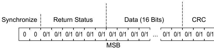
Figure 31: Manchester Read Response
