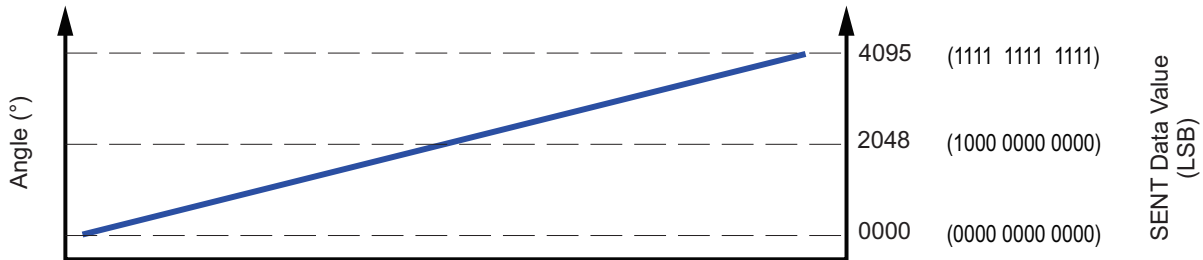
Figure 38: Angle is Represented as a 12-bit Digital Value
