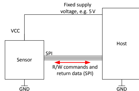
Figure 16: SPI Interface Programming Setup
