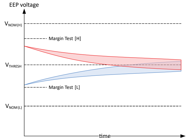
Figure 35: Example of Failing Programming Voltages
