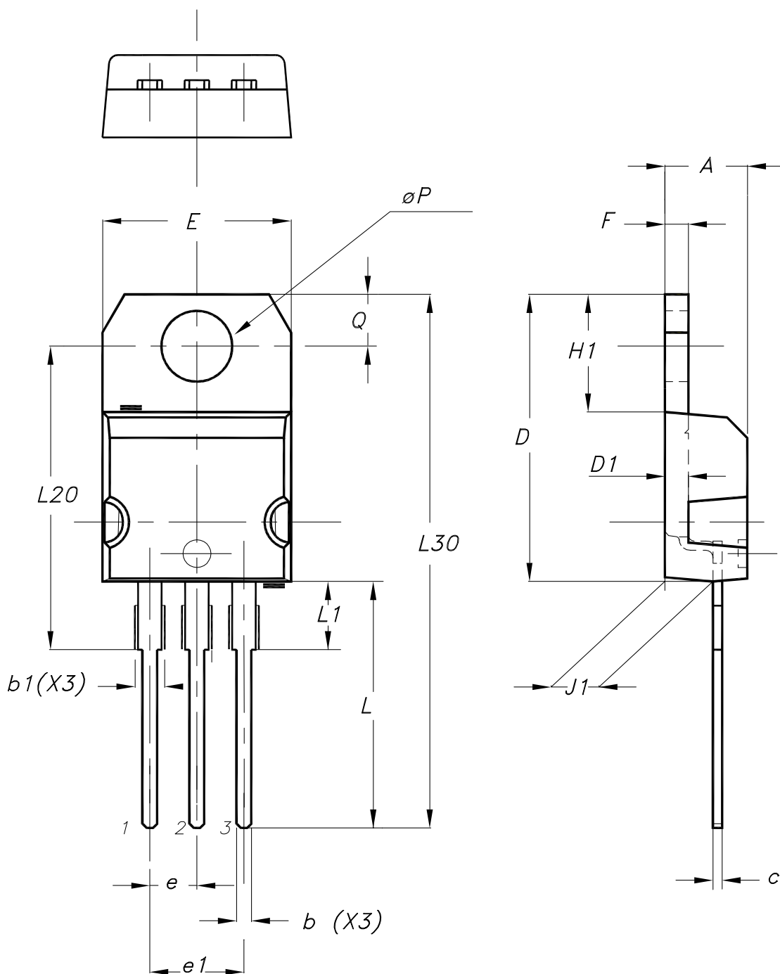
Figure 9. TO-220AB package outline
