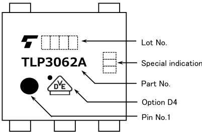
Fig. 16.3 Marking Example of TLP3062A(Note)
