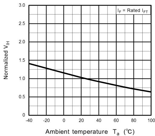
Fig. 12.12 Normalized V_H - T_a
