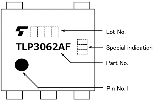
Fig. 15.1 Marking Example of TLP3062A(Note) Fig. 15.2 Marking Example of TLP3062AF(Note)
