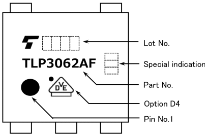
Fig. 16.4 Marking Example of TLP 3062AF (Note)
