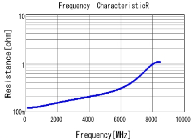
■ GCQ1555C1H4R4BB01 R DC0V, 25degC
