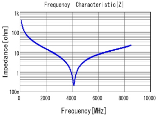
■ GCQ1555C1H4R4BB01 |Z| DC0V, 25degC
