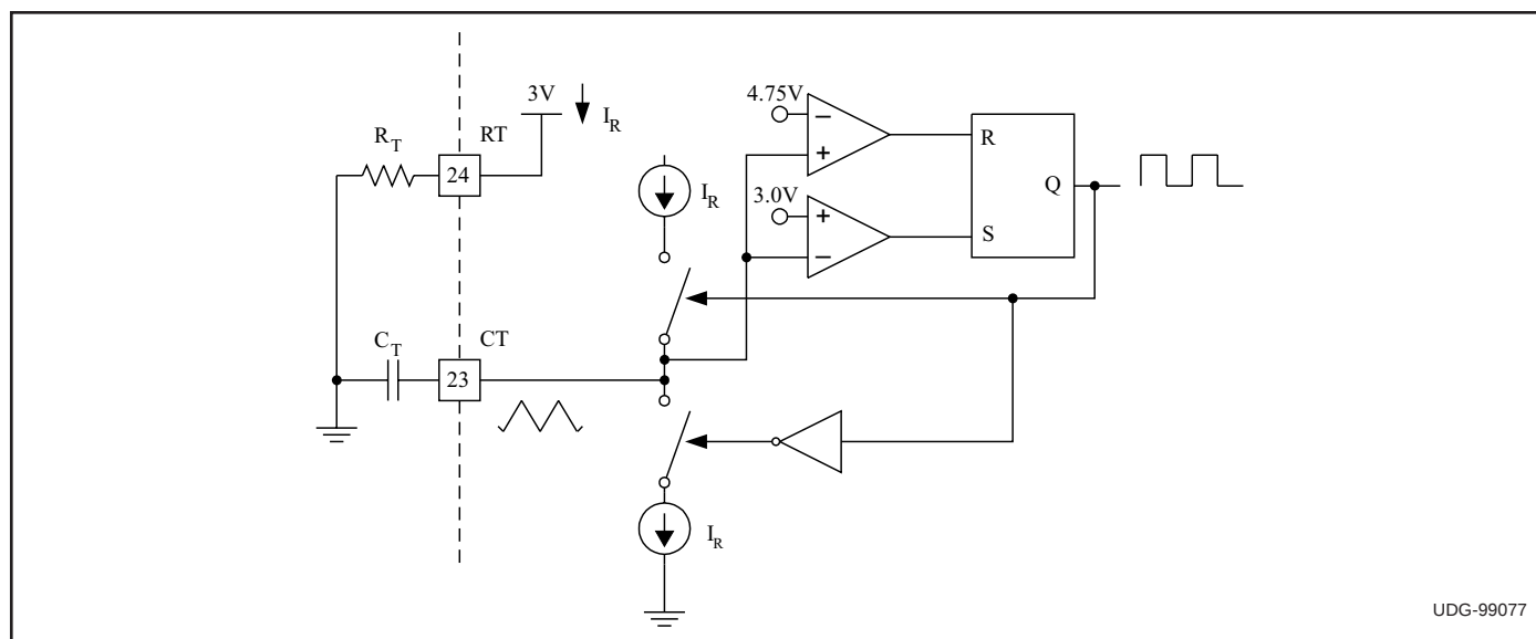
Figure 7. Oscillator setup.
