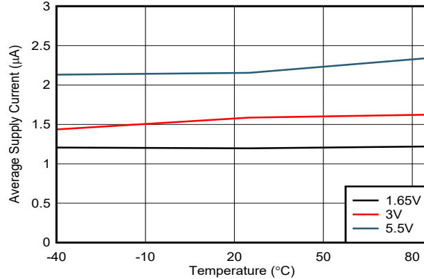
Figure 6-1. I_{CC(AVG)} vs Temperature (20-Hz versions)
