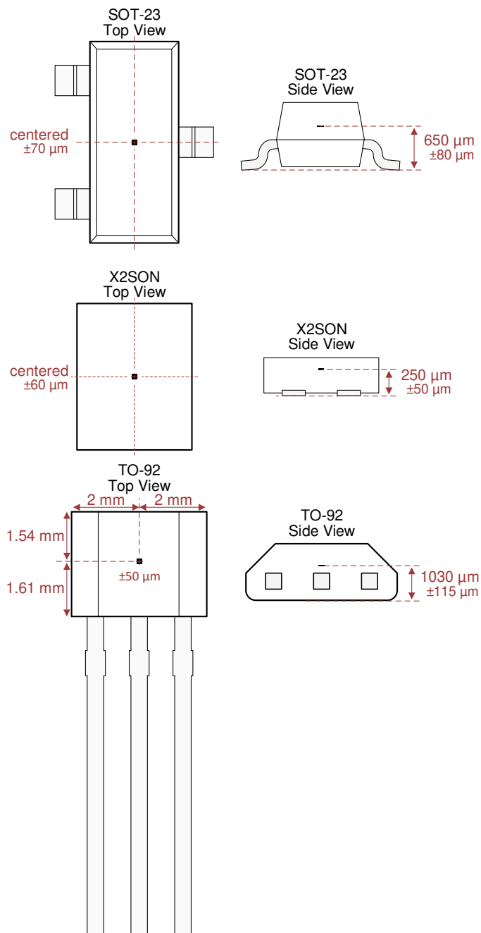
Figure 7-8. Hall Element Location
