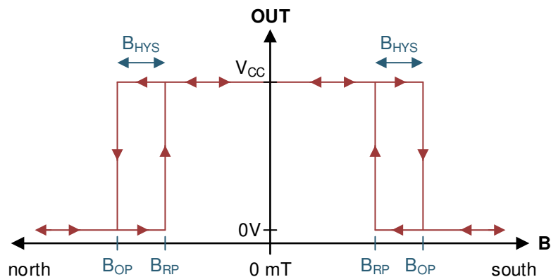
Figure 7-3. Omnipolar Functionality
