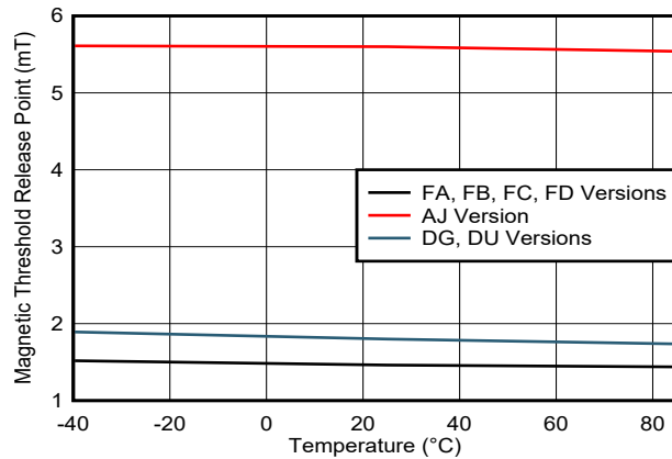
Figure 6-5. |B_{RP}| vs Temperature
