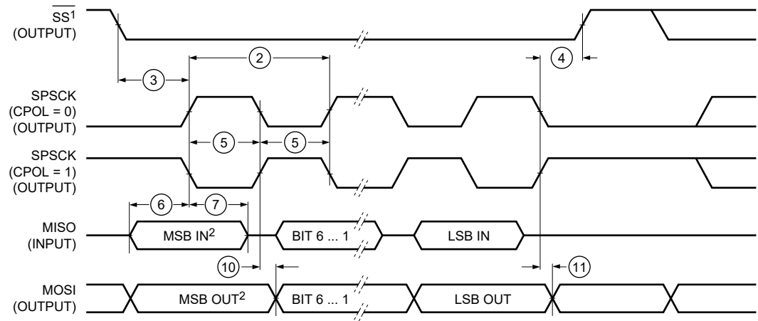
Figure 50. LPSPI Controller Mode Timing (CPHA=0)
