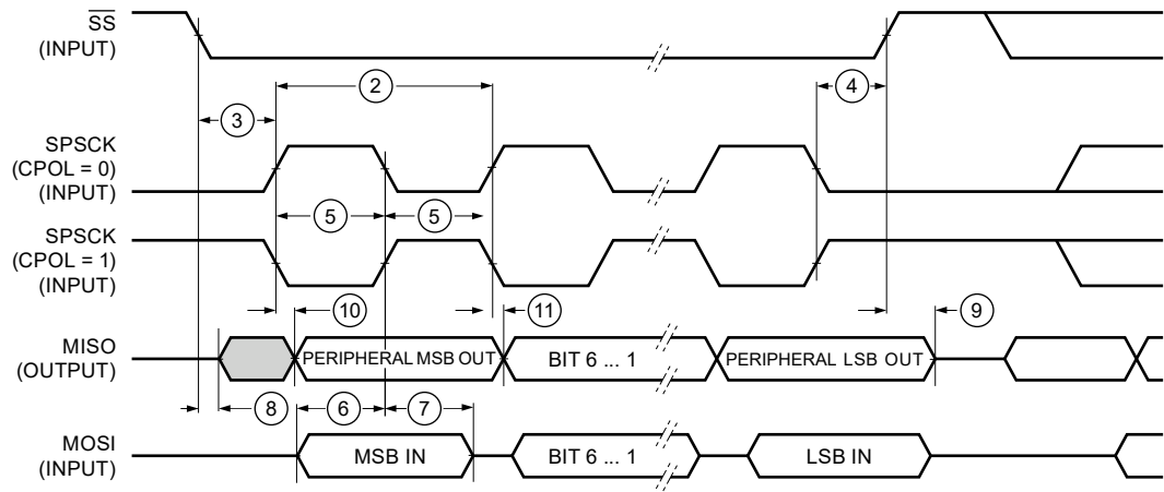
Figure 48. LPSPI Peripheral Mode Timing (CPHA=1)
