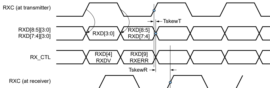
Figure 61. RGMII Receive Timing
