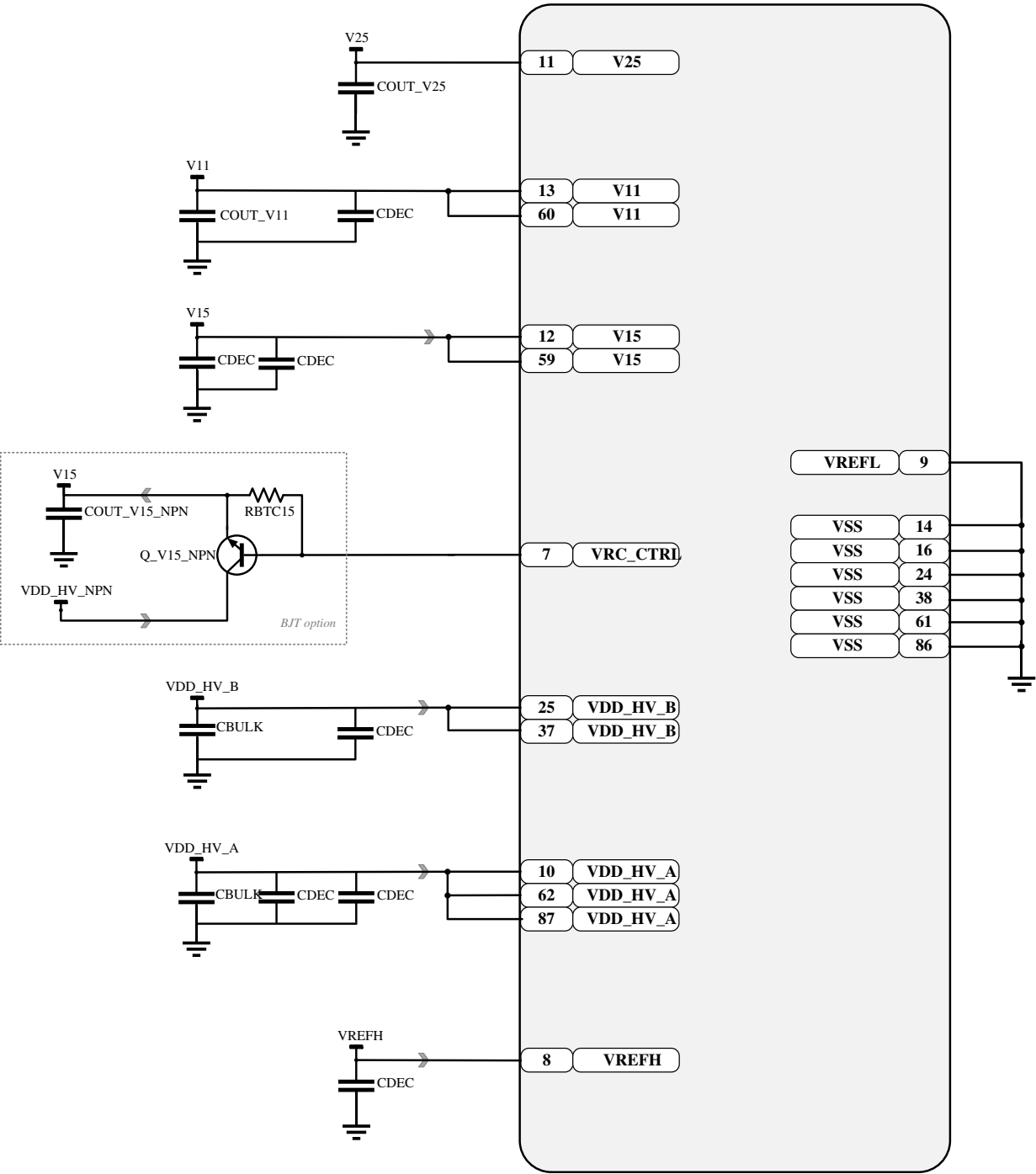
Figure 32. 100LQFP package decoupling capacitor pinout diagram, (S32K344, S32K324, S32K314)
