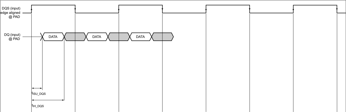
Figure 66. QuadSPI Input timing (DDR mode)
