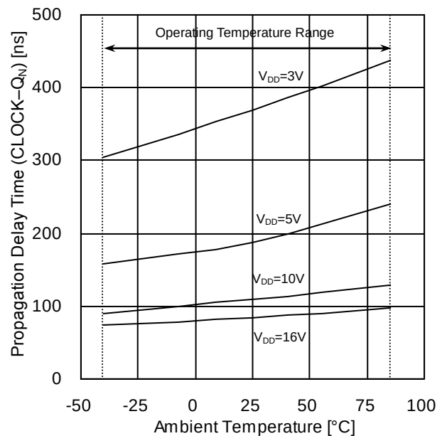
Figure 8. Propagation Delay Time t_{PLH} (CLOCK-Q N ) vs Ambient Temperature
