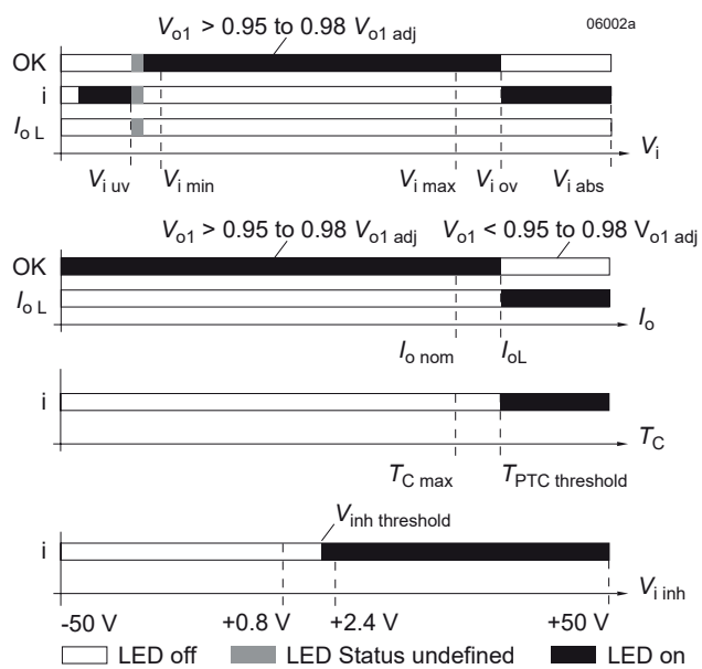
Fig. 12 LED indicators
