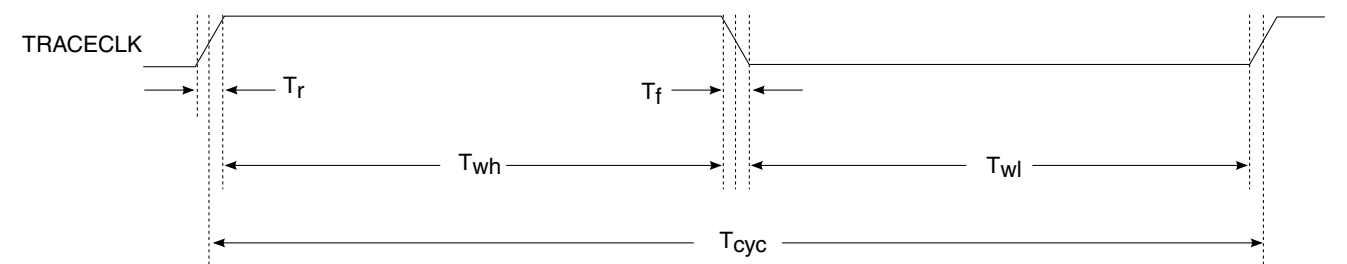
Figure 57. TRACE_CLKOUT specifications
