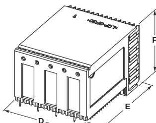
Plug (Daughtercard)
