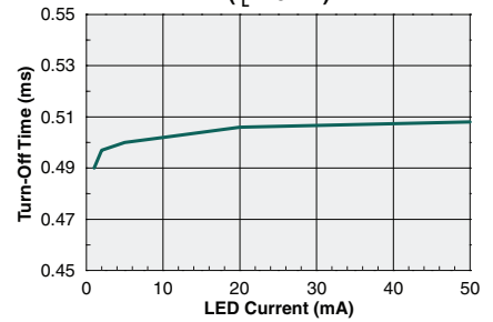
Typical Turn-Off Time vs. LED Forward Current ( I_L=70\text{mA} )
