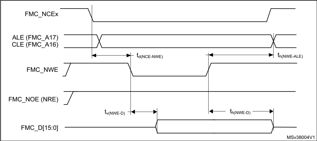
Figure 55. NAND controller waveforms for write access
