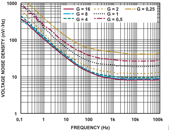
Figure 30. Input Referred Voltage Noise Density vs. Frequency
