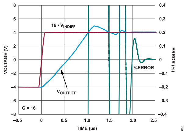
Figure 59. Settling Time to 8 V p-p Output Step
