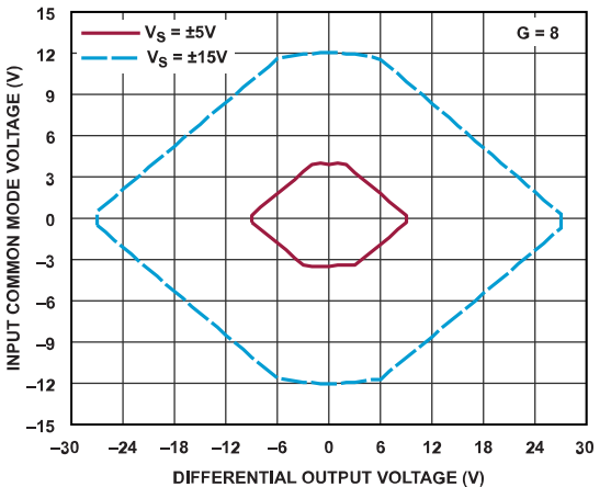
Figure 79. Input Common Mode Range vs. Differential Output Voltage at G = 8 with No Load
