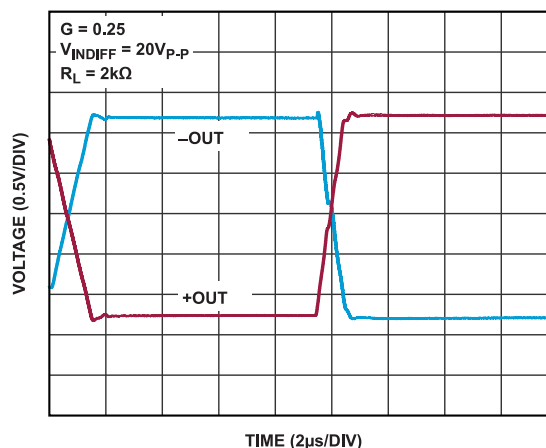
Figure 54. Large Signal Step Response
