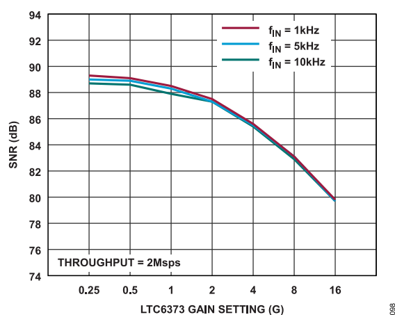
Figure 97. SNR for LTC6373 Driving ADAQ4003 (Gain = 0.9)
