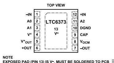
Figure 2. Pin Configuration
