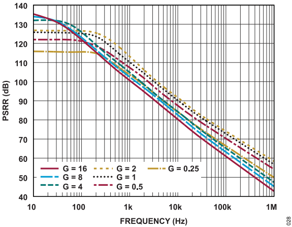
Figure 27. Negative PSRR vs. Frequency, RTI
