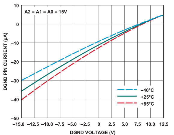
Figure 38. DGND Pin Current vs. DGND Pin Voltage
