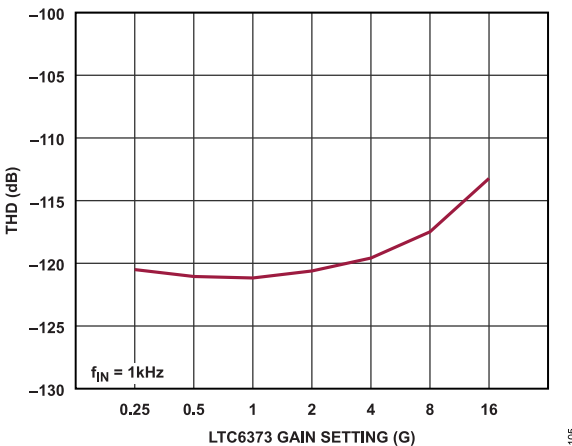
Figure 104. THD for LTC6373 + ADA4945-1 + AD7768-1 Signal Chain
