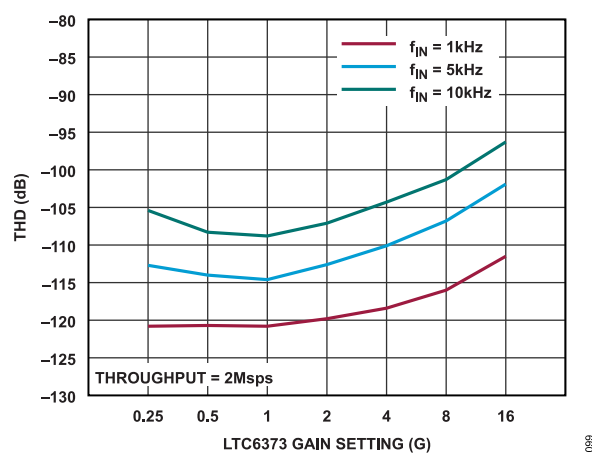
Figure 98. THD for LTC6373 Driving ADAQ4003 (Gain = 0.9)
