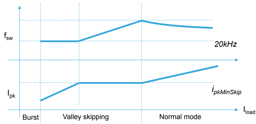
Figure 9. Transition between normal mode, skip mode and burst mode
