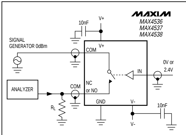
Figure 4. Off Isolation
