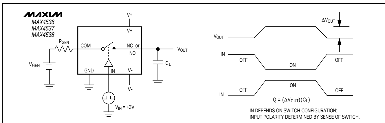
Figure 3. Charge Injection
